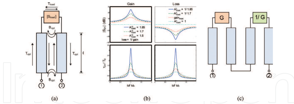
Figure 4. Proposed active reconfigurable all-pass phaser by cascading a gain-loss pair. (a) Loaded C-section [35] and (b) amplitude |S_{21}| and normalized group delay \tau_{21}/T_0 of the gain/loss loaded C-section, where the coupling factor k = 0.5 at \omega_0 . (c) Loss-gain all-pass C-section pair. ©IEEE; reprinted with permission.
