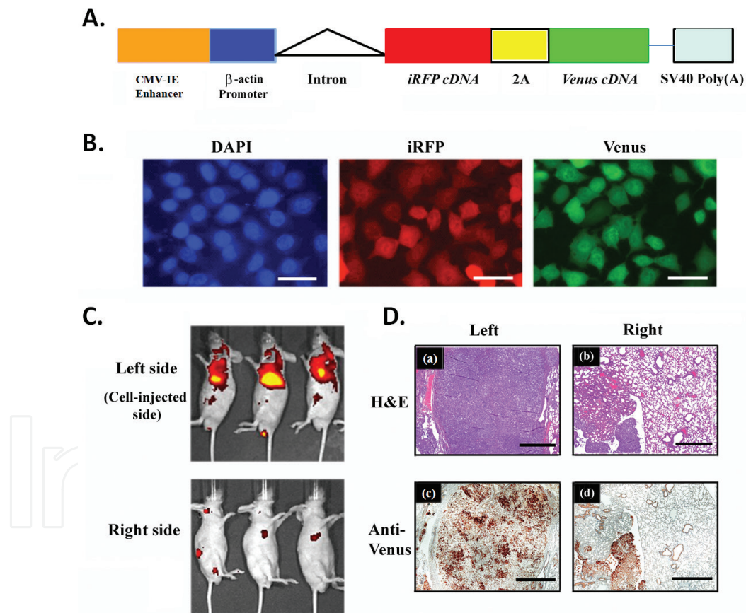
Figure 2. Animal model 2 for dual fluorescence reporting genes expressed by in vivo imaging model of orthotopic lung adenocarcinoma in mice. (A) Construction map of dual fluorescence expression vector, pCAG-iRFP-2A-venus transgene. (B) Three different fluorescence signals were used in iRFP-2A-Venus A549 cells expressed under a fluorescent microscope: DAPI (blue), iRFP (red) and venus (green). Scale bar: 50 \mu m. (C) The IVIS imaging analysis of nude mice that received iRFP-2A-venus A549 cells by orthotopic injection. Color scale: Max: 4.56e+7 , Min: 2.02e+7 . (D) Histopathologic study of nude mice lung tumors after receiving iRFP-2A-venus A549 cells by orthotopic injection. L and R represent left and right lungs, respectively. The left side column (a) and (c) represent H&E and IHC expression on the longitudinal sections of lung tumors, respectively. The brown color of antivenus expression in column (c) and (d) indicates lung tumor formation. The scale bar in columns (b) and (d) is 100 \mu m.
