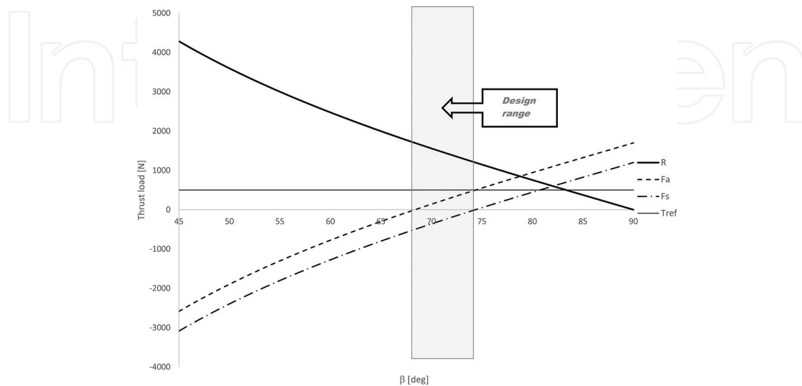
Figure 11. Trends of axial bearing thrusts and load transfer as a function of helix angle in nominal operating conditions.
