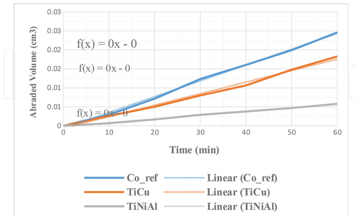
Figure 10. Abraded volume vs. time for the tested metallic matrices during abrasion test.
