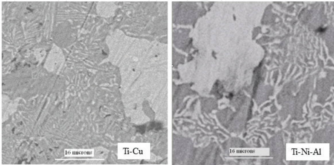
Figure 3. Optical microstructures of the investigated metallic matrices.
