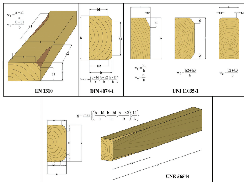
Figure 5. Width of the wane according to European visual strength grading standards ( w_e = wane on edge, w_f = wane on face).
