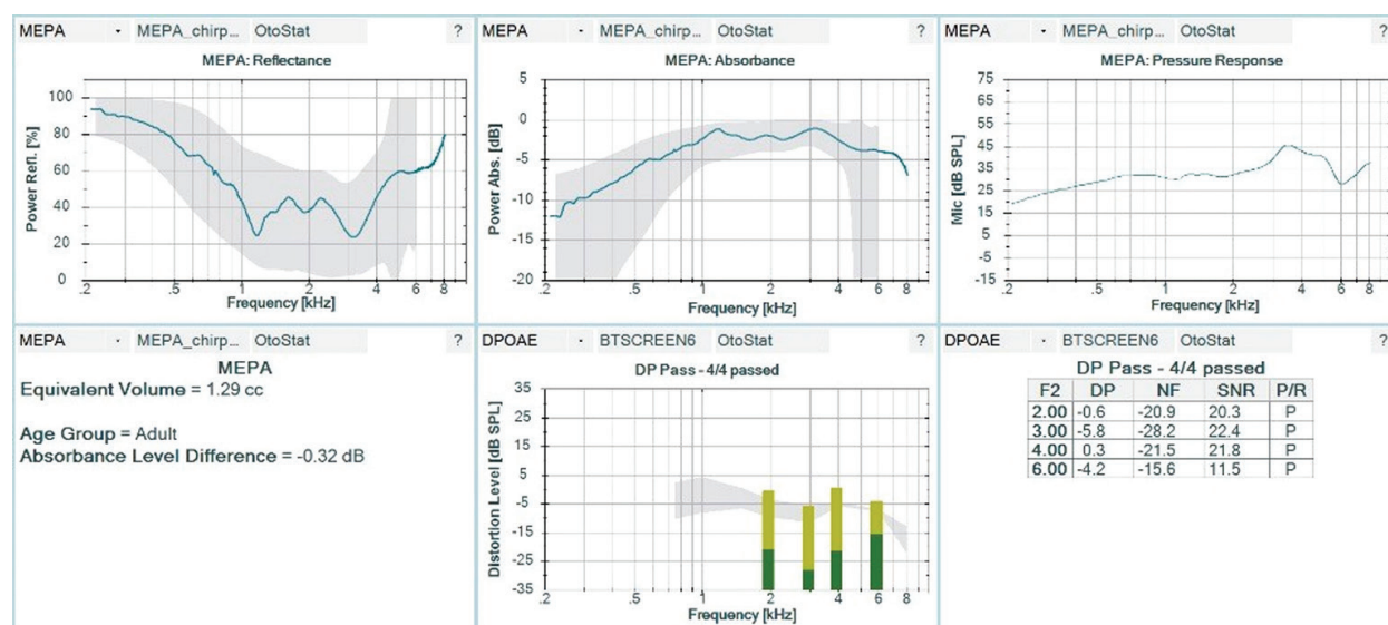
Figure 2. WBT data from the Otostat system (Mimoso Acoustics). The panels indicate WBT reflectance, absorbance, and pressure response \times tested frequency (the Otostat uses a chirp stimulus). The lower panels show the distortion product OAEs in terms of spectrum and S/N ratios at the four tested frequencies. The WBT + OAE combination favors a good assessment of the ME function in neonates, and it can be used to avoid many REFER or FAIL results.
