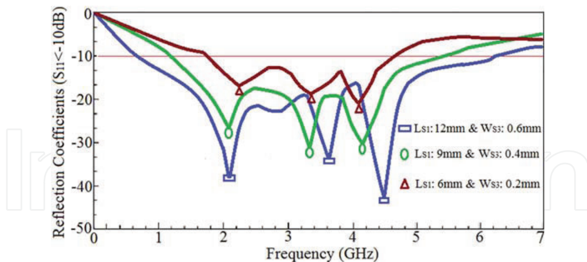
Figure 12. Effect on the antenna impedance bandwidth as a function of H-slit length ( L_{S1} ) and width ( W_{S3} ). All other structural parameters given in Table 1 remain fixed.
