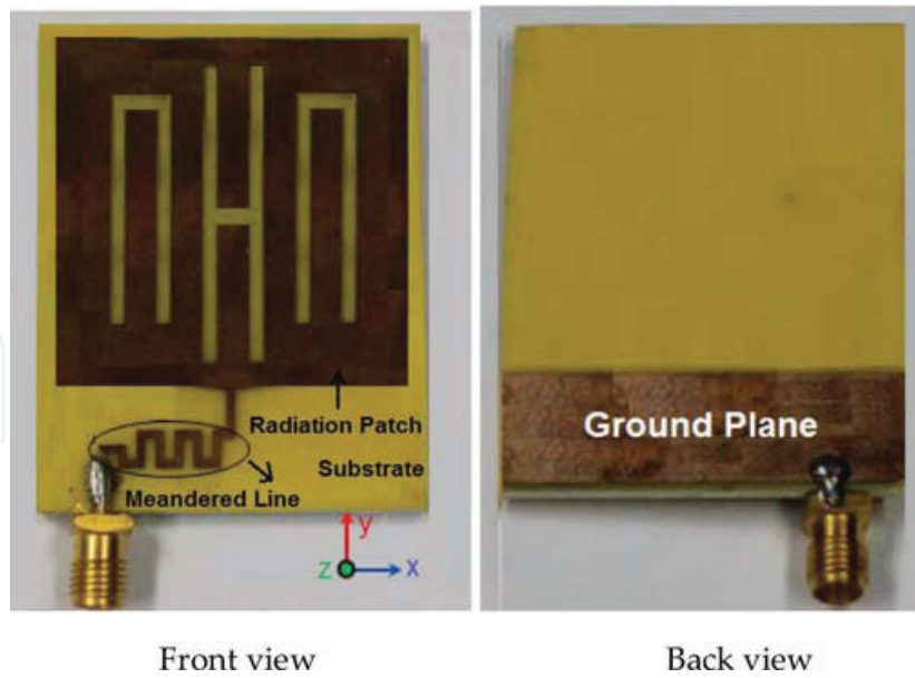
Figure 6. Fabricated prototype MTM antenna.
