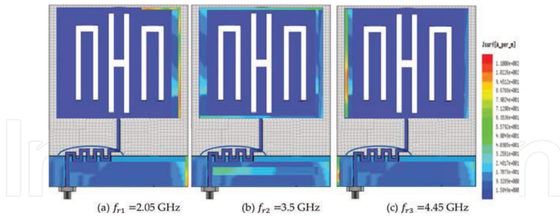
Figure 11. Current density distribution over the MTM antenna at various spot frequencies. (a) f_{r1} = 2.05 GHz; (b) f_{r2} = 3.5 GHz; (c) f_{r3} = 4.45 GHz.
