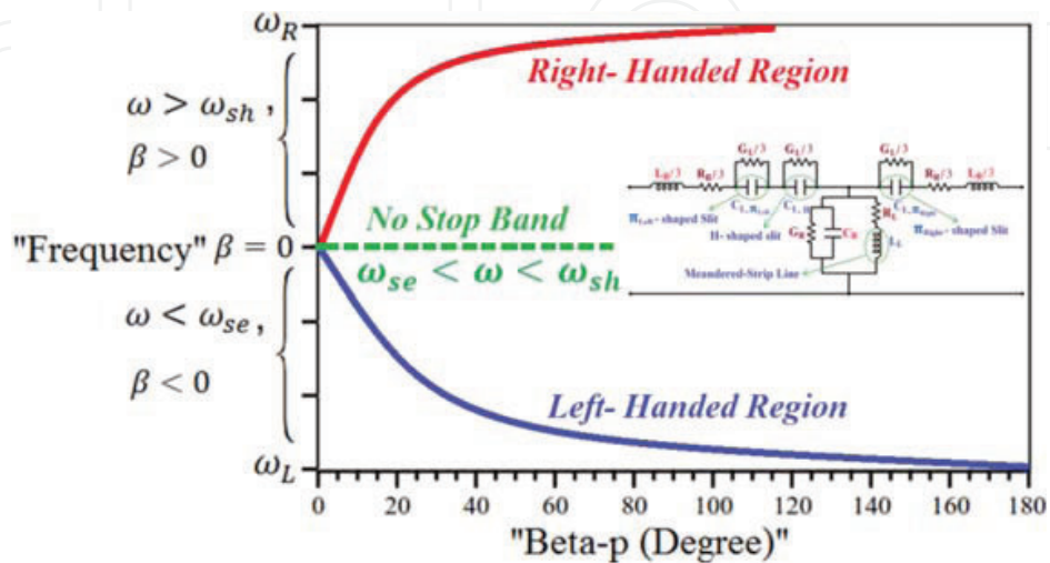
Figure 7. Dispersion diagram.
