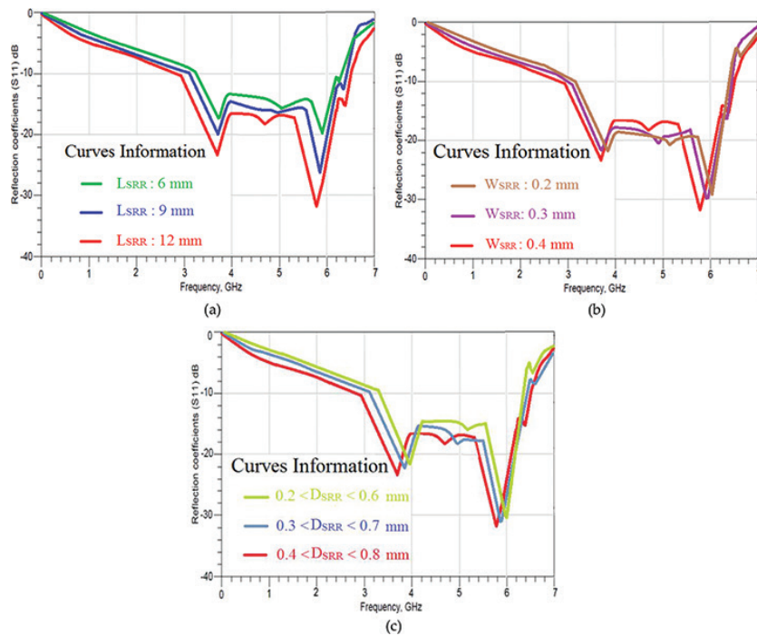
Figure 10. Parametric study on SRR dimensions for the F-shaped antenna. (a) Effect of SRR length ( L_c ) (all other parameters remain constant). (b) Effect of SRR width ( W_s ) (all other parameters remain constant). (c) Effect of gap between the rings of the SRR ( D_{SRR} ) (all other parameters remain constant).
