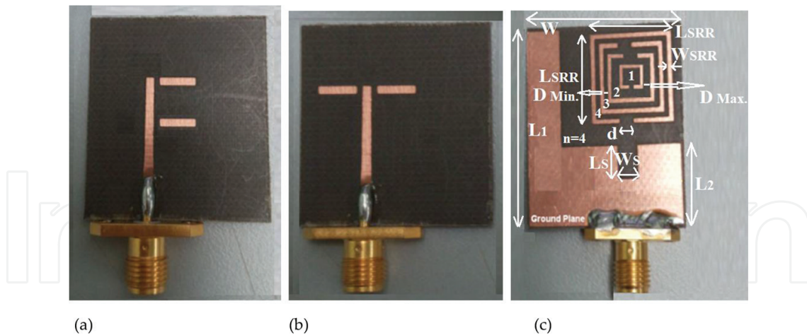
Figure 2. Fabricated prototypes of the antennas with asymmetrical SRR loading, (a) top view of F-shaped antenna, (b) top view of T-shaped antenna, and (c) back view of both antennas with SRR loading.
