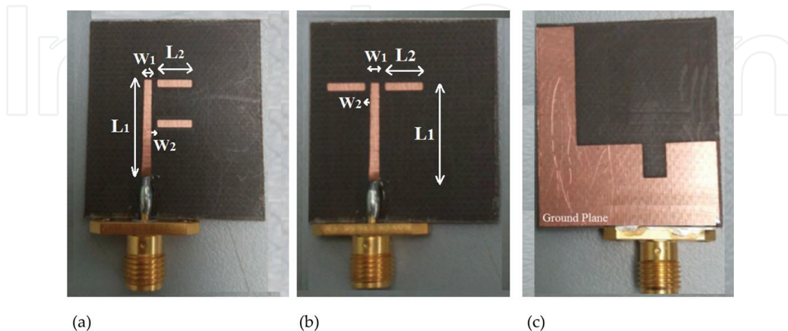
Figure 1. Fabricated prototypes of the monopole antennas, (a) top view of F-shaped antenna, (b) top view of T-shaped antenna, and (c) back view of both antennas without SRR loading. The antennas are in the xy plane.
