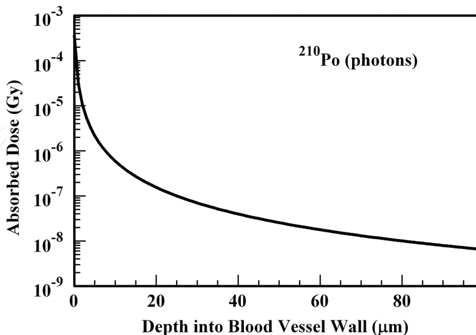
Figure 3. Absorbed dose profile for ^{210}\text{Po} photons in a water medium. The absorbed dose is delivered by 0.3 Bq of ^{210}\text{Po} uniformly deposited within a 1- \mu\text{m} -diameter microsphere following the total decay of the radioactive material.
