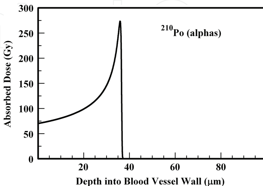
Figure 2. Absorbed dose profile for ^{210}\text{Po} alpha particles in a water medium. The absorbed dose is delivered by 0.3 Bq of ^{210}\text{Po} uniformly deposited within a 1- \mu\text{m} -diameter microsphere following the total decay of the radioactive material.
