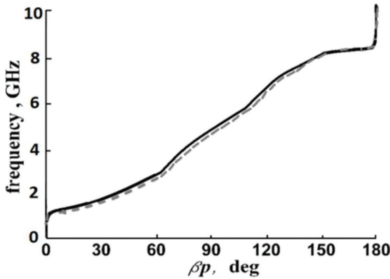
Figure 3. Dispersion diagram of the proposed antenna constructed using SCRLH-TL. HFSS™ (solid line) and Eq. (6) (dashed line).
