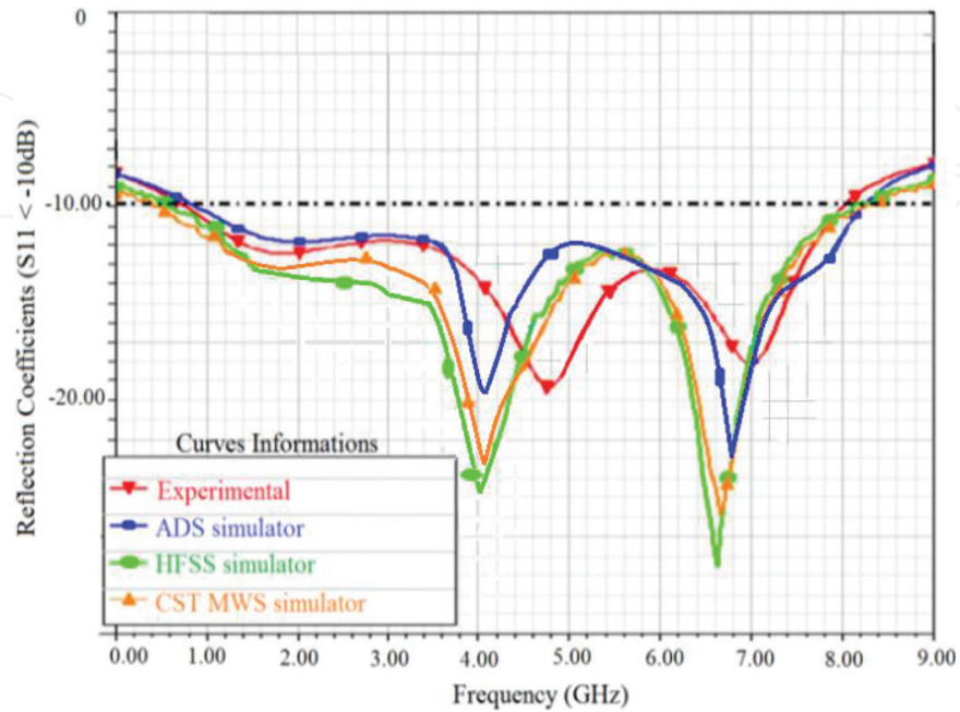
Figure 5. Antenna measured and simulated reflection coefficient response.
