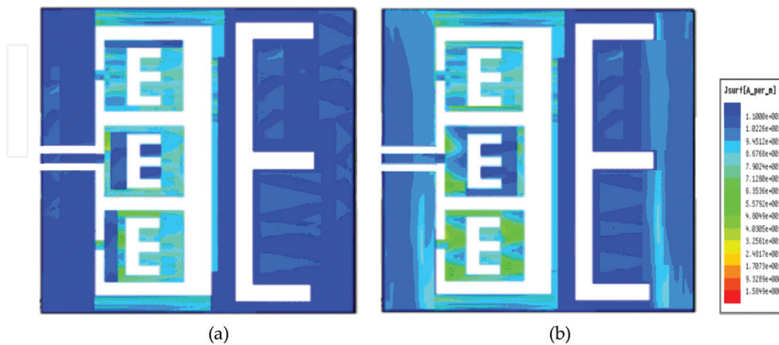
Figure 6. Current density distribution over the antenna at (a) 4.75 GHz and (b) 7 GHz.
