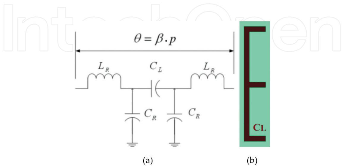
Figure 2. Simplified CRLH structure without inductance L_L : (a) lumped structure and (b) distributed equivalent one.
