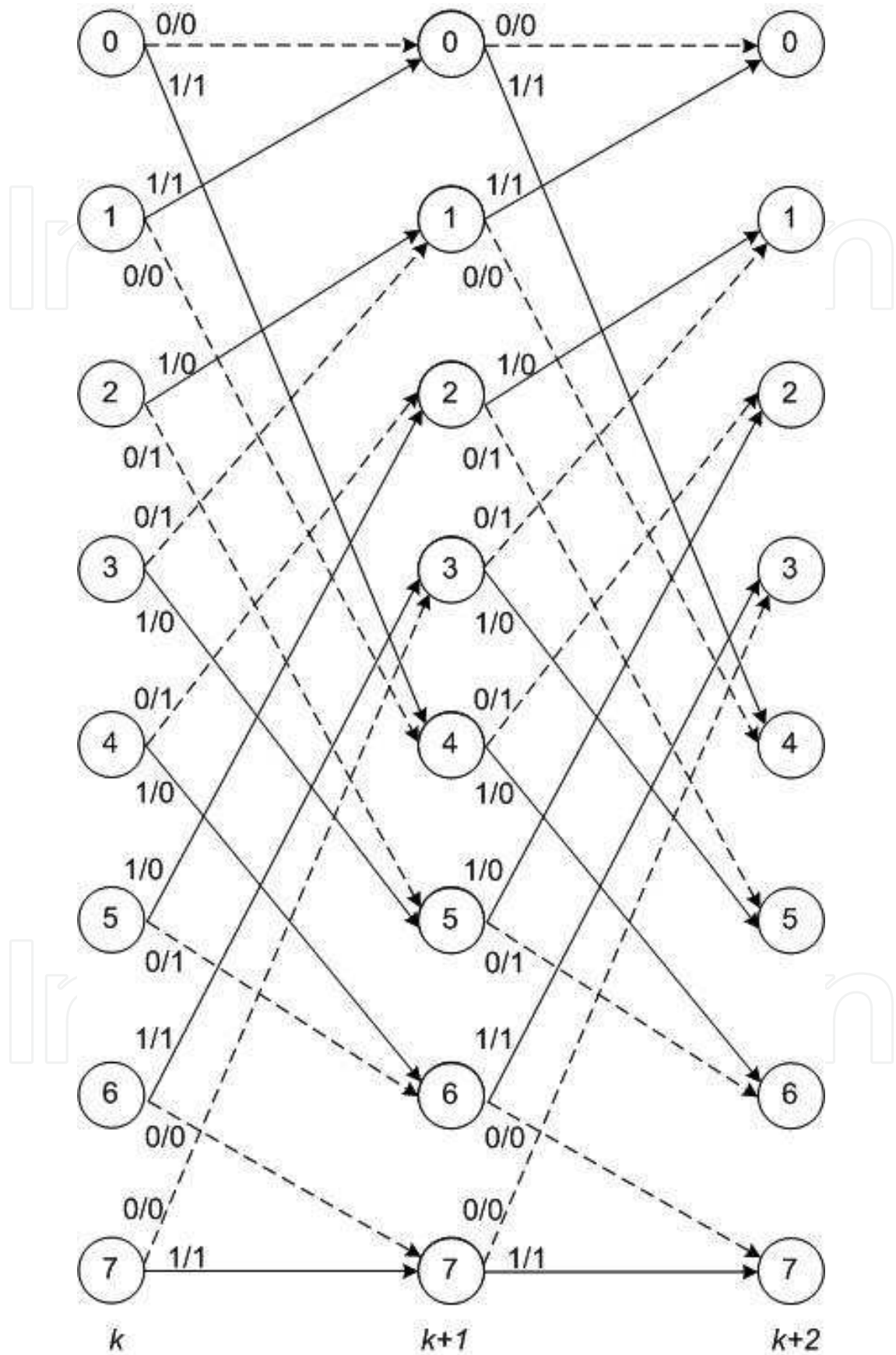
Figure 6. LTE turbo coder trellis.
