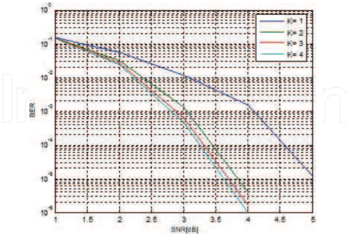
Figure 16. The impact of the number of iterations on decoding performances.
