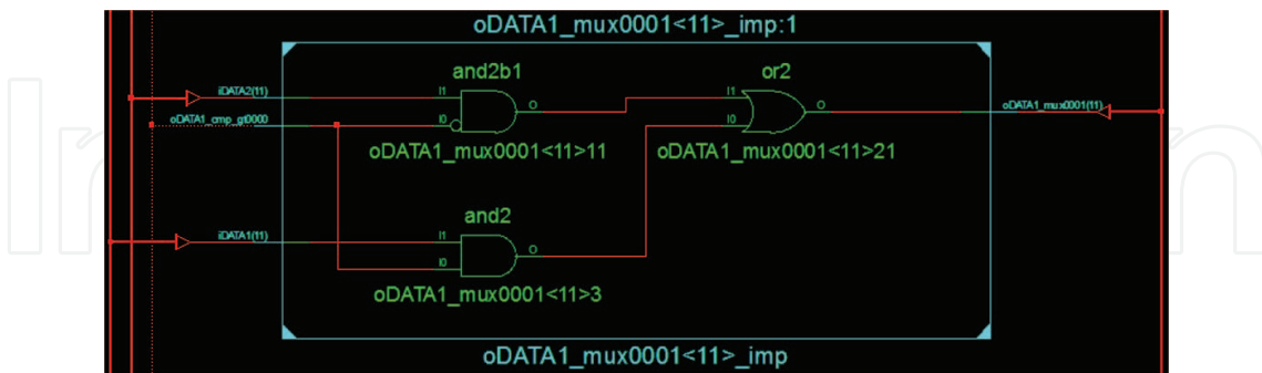
Figure 18. Basic selection element for binary inputs.
