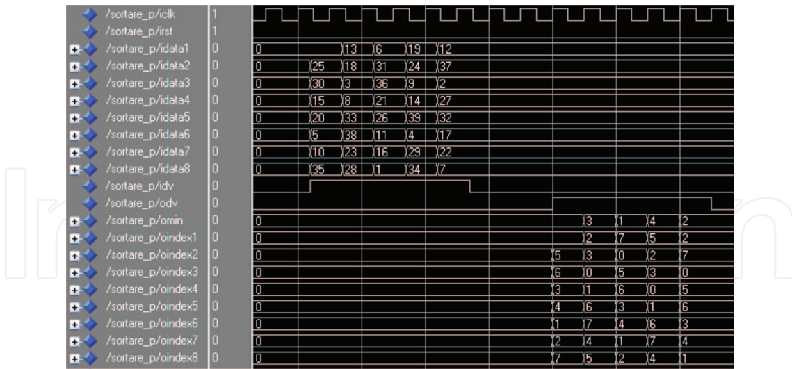
Figure 19. Even-odd merge sort – ModelSim simulation.
