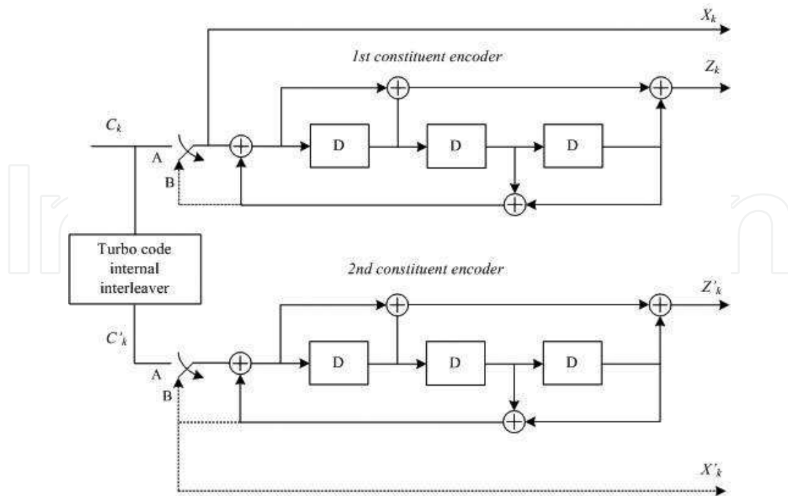
Figure 2. LTE turbo coding scheme.
