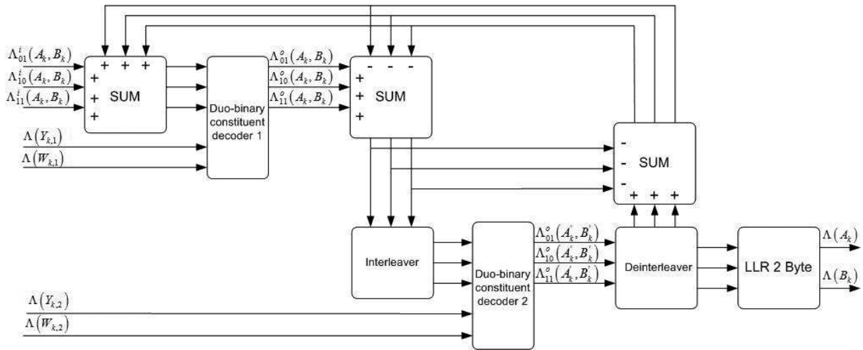
Figure 4. Decoder block scheme.
