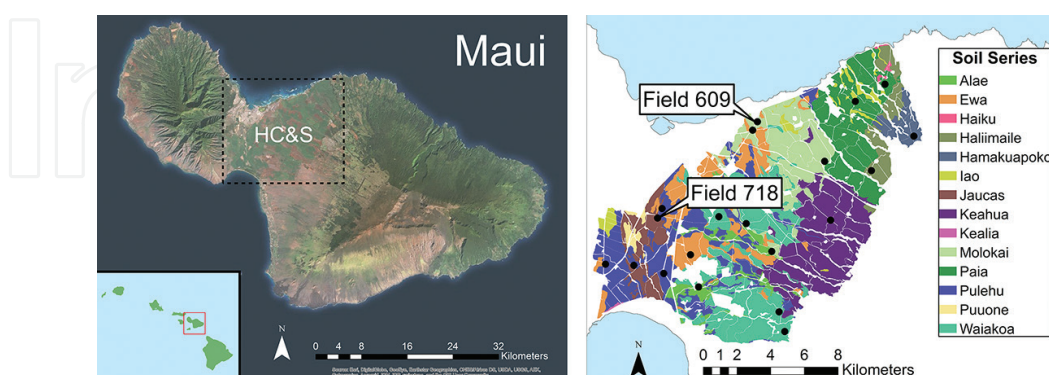
Figure 1. Maui with the main Hawaiian Islands inset (left) and Hawaiian Commercial & Sugar Company fields and associated soil series (right). Soil series data from: Soil Survey Staff, Natural Resources Conservation Service, United States Department of Agriculture. Web Soil Survey. Available online at http://websoilsurvey.nrcs.usda.gov/ . Accessed [07/30/2016].
