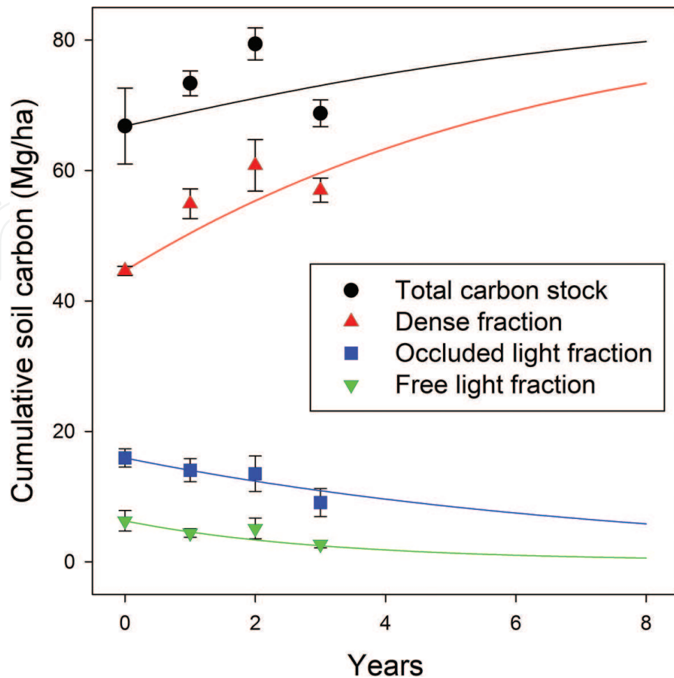
Figure 6. Three-pool model completed in SoilR (R project package, [32]) using density fractionation and measured ESM soil stock data from field 718 under ratoon harvest energy cane and zero-tillage. An ESM reference mass of 3600, which represents the shallowest mass soil depth was used for C stocks (Figure 5). Pool fraction data was determined from 0 to 20 cm depth samples (same cores ESM carbon stocks were calculated from).
