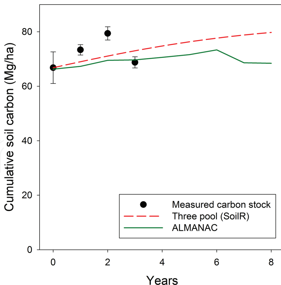
Figure 9. Two models (ALMANAC and SoilR) projected forward from surface soil (ESM 3600) for 8 years compared to measured data.
