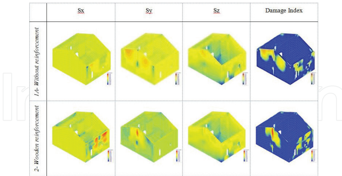
Figure 7. Dynamic-seismic method.
