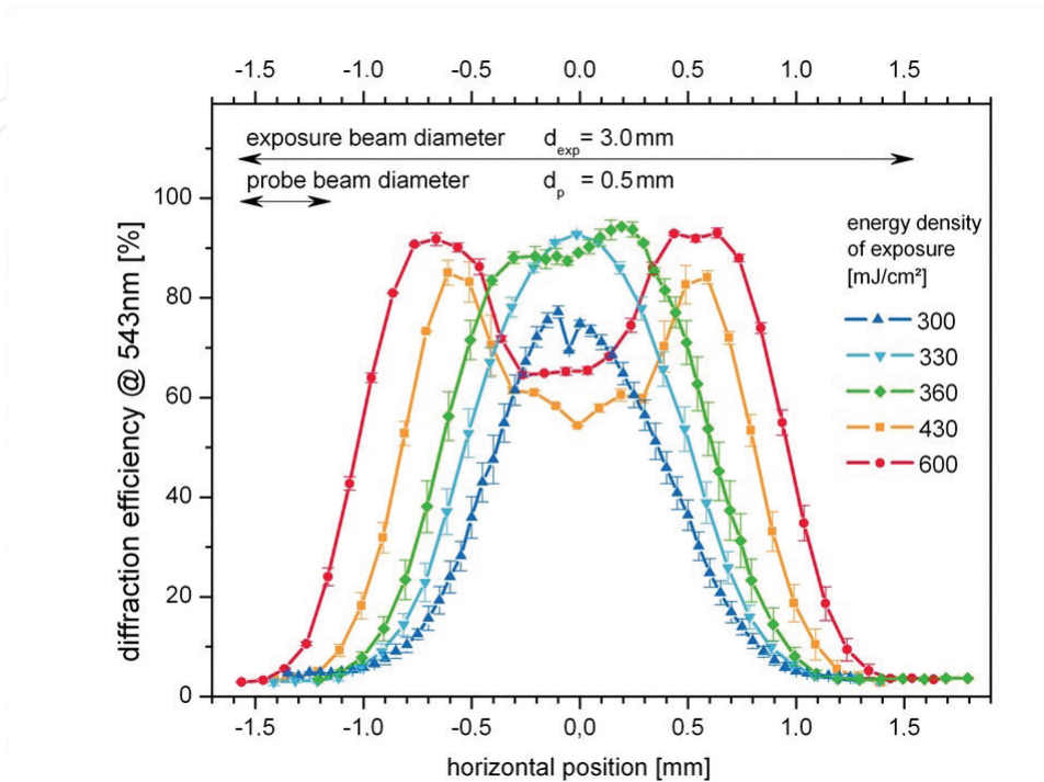
Figure 9. Principle of lateral scanning: Holograms were recorded with exposure beam diameter of 3mm and scanned step-by-step with a probe beam diameter of 0.5 mm. Five lateral scans are shown. The corresponding gratings were recorded with different exposure energy densities.
