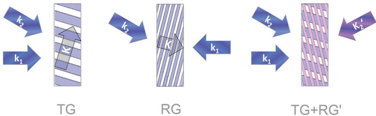
Figure 3. Recording geometries for transmission grating (TG) and reflection grating (RG). Wave vectors of recording beams \vec{k} as well as grating vectors \vec{K} are displayed. The reflected wave forms a secondary grating (RG') [5].
