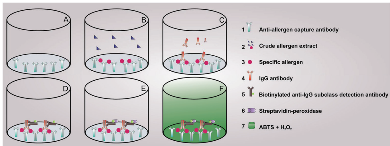
Figure 3. Representative diagram (sequential steps A to F) of the reverse enzyme-linked immunosorbent assay (ELISA). (1) Capture allergen-specific (Der p 1 or Der p 2) monoclonal antibody; (2) crude Dermatophagoides pteronyssinus extract; (3) allergen (Der p 1 or Der p 2) present in crude extract; (4) allergen-specific IgG antibody present in serum samples or other biological fluids from allergic patients; (5) monoclonal antibody against human IgG subclass (preferentially IgG4) labeled with biotin; (6) streptavidin-peroxidase enzymatic conjugate; (7) reaction is revealed by the addition of enzymatic substrate (hydrogen peroxide) diluted in a chromogenic buffer (ABTS) and absorbance is determined in a plate reader at 405 nm (Taketomi EA and Silva DAO, 2016, found in European Patent Office EP 2232265 [68]).
