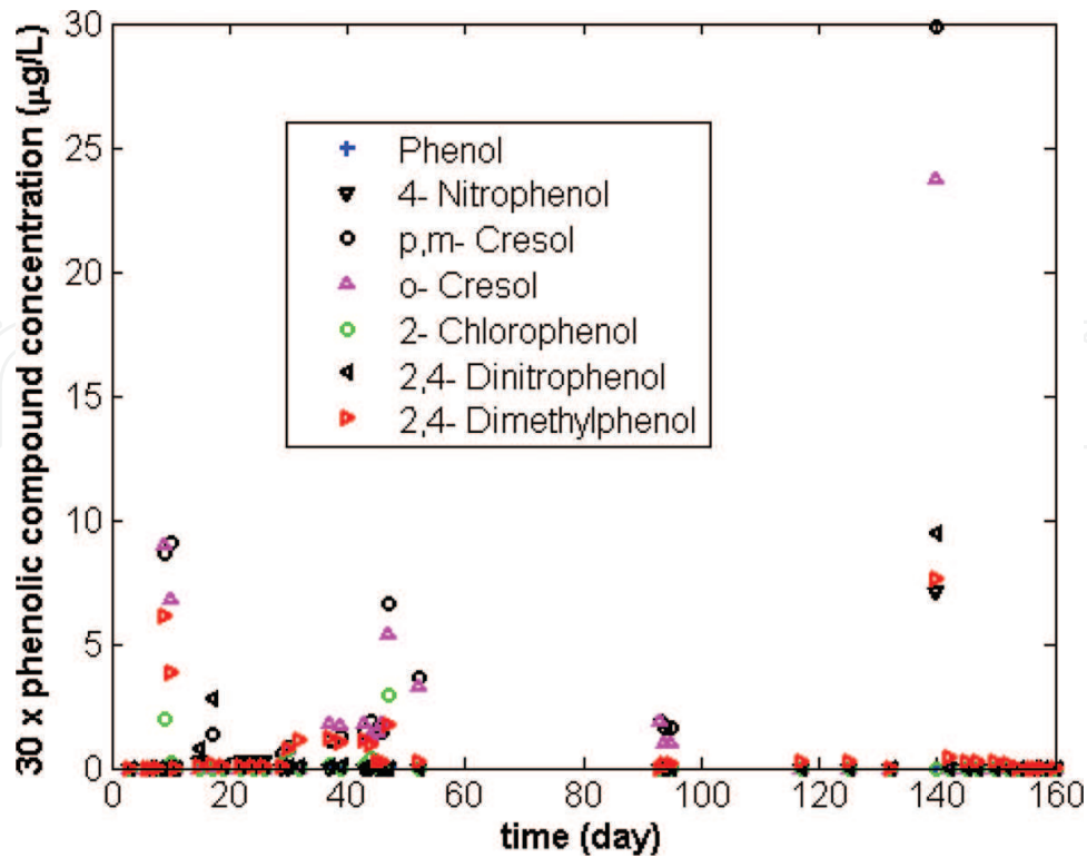
Figure 8. Phenolic compounds profiles variation in the column 2 (biofilter).
