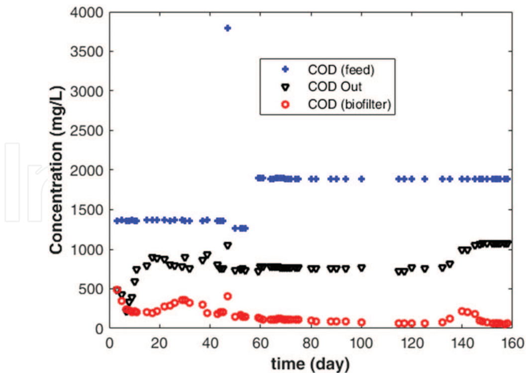
Figure 12. COD profiles comparison in woodwate leachate influent and in both columns with and without bacterial activity.
