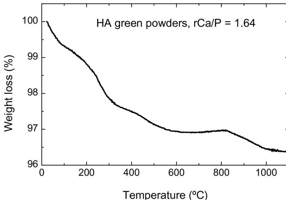
Figure 2. TGA of as-prepared HA green powders.
