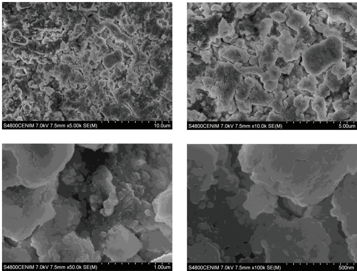
Figure 6. SEM micrographs under different magnifications of HA-2 powders prepared using CRTA ( T_m = 300^\circ\text{C} ).
