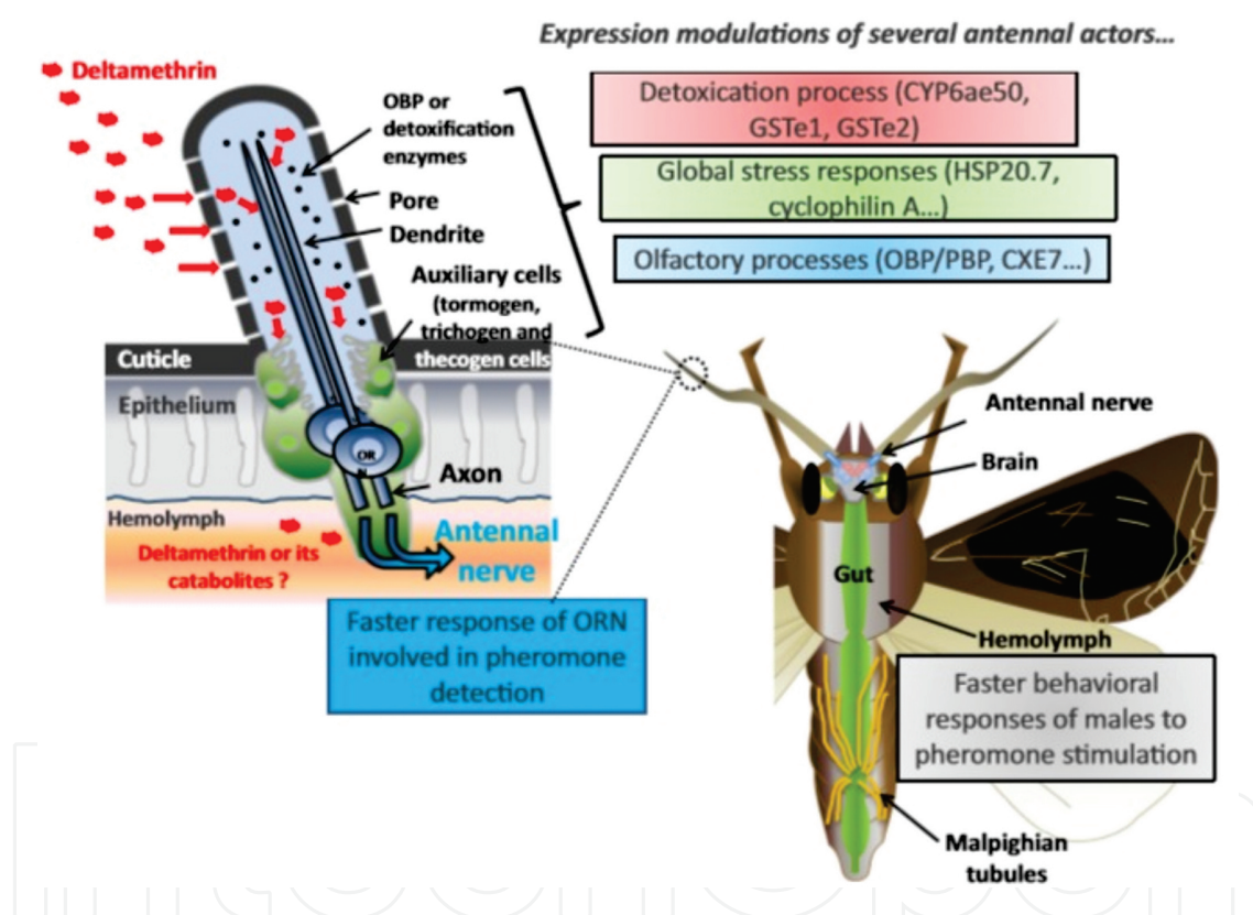
Figure 1. Proposed effect model of sublethal doses of deltamethrin upon Spodoptera littoralis (Boisduval) (Lepidoptera: Noctuidae) olfactory system [23].
