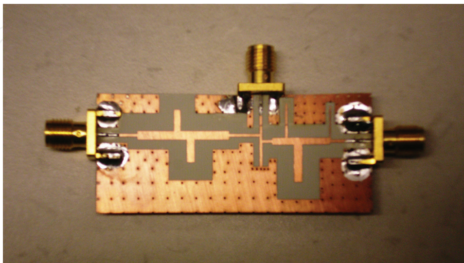
Figure 15. Prototype of FDN.
