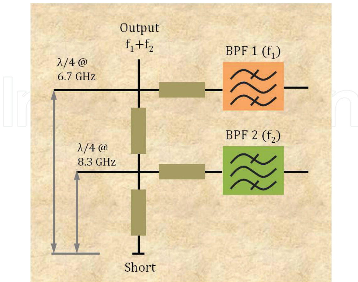
Figure 8. Frequency diplexer network [21].
