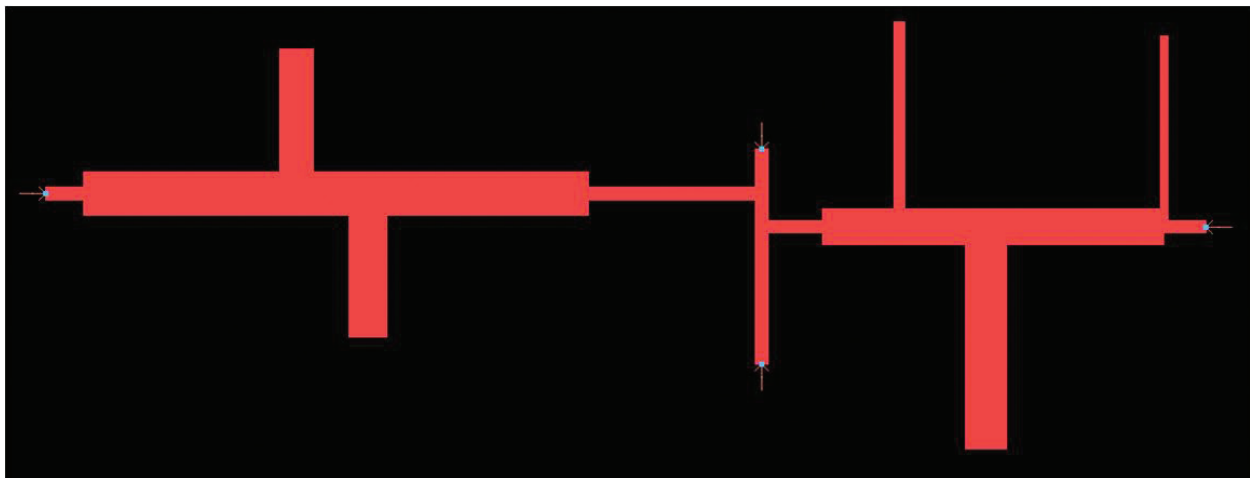
Figure 11. Layout of the FDN.
