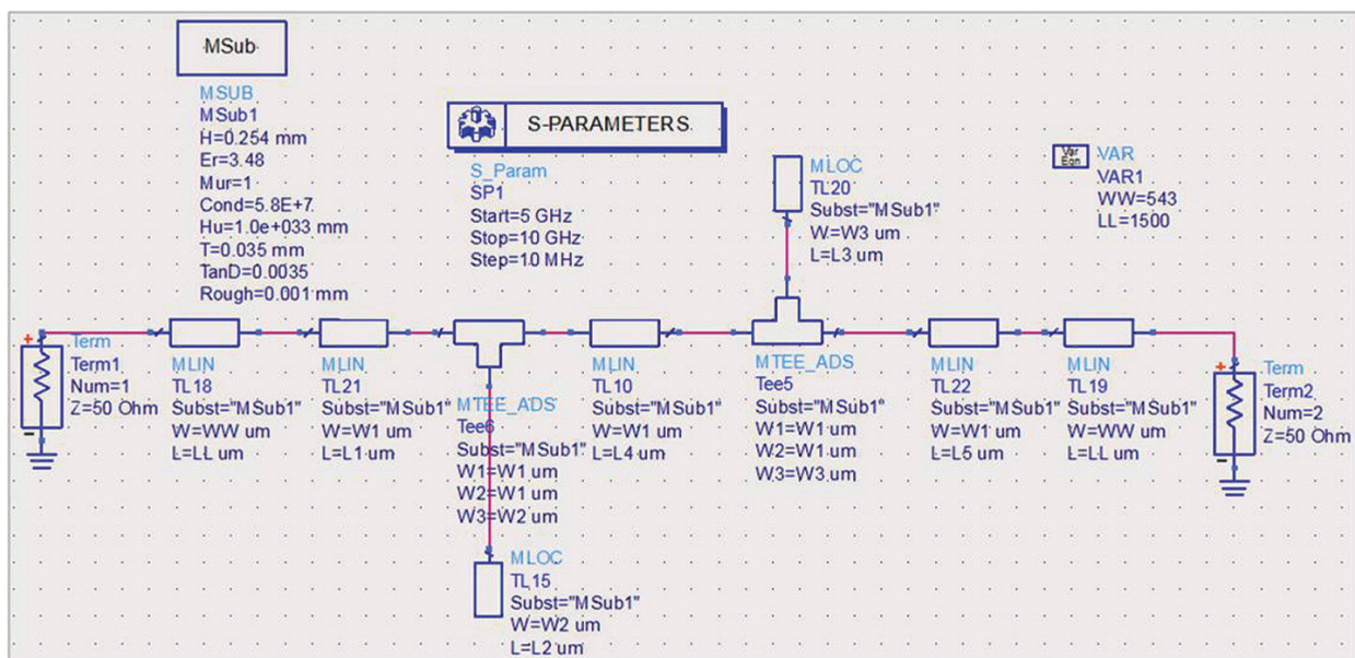
Figure 9. Schematic diagram of first filter for 6–7.4 GHz.
