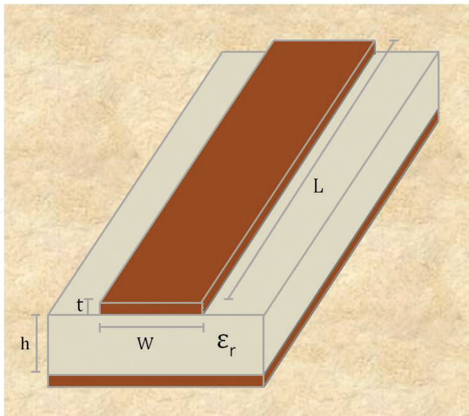
Figure 5. Microstrip transmission line.
