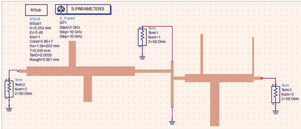
Figure 12. FDN as layout component in schematic representation.
