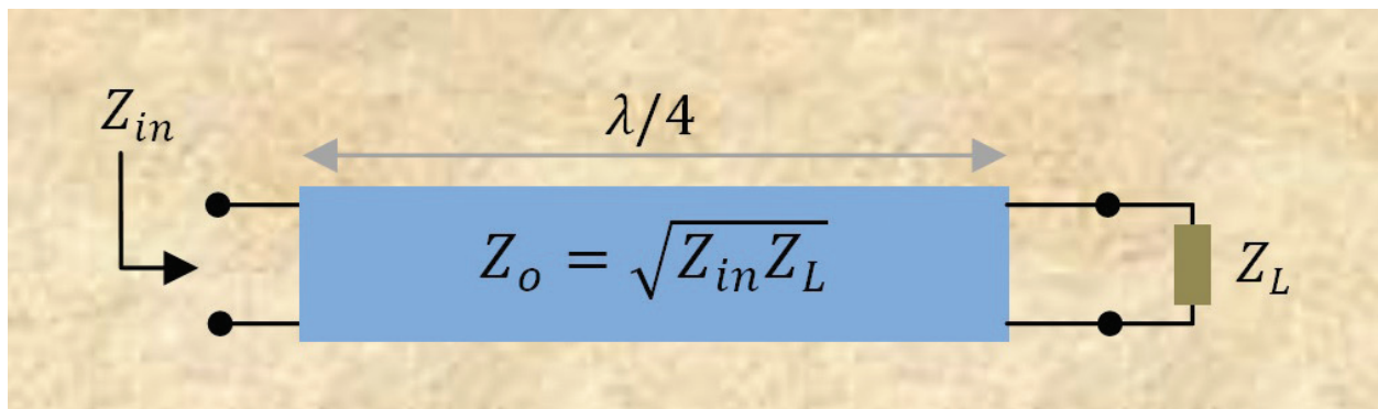
Figure 6. Quarter wavelength microstrip transmission line.
