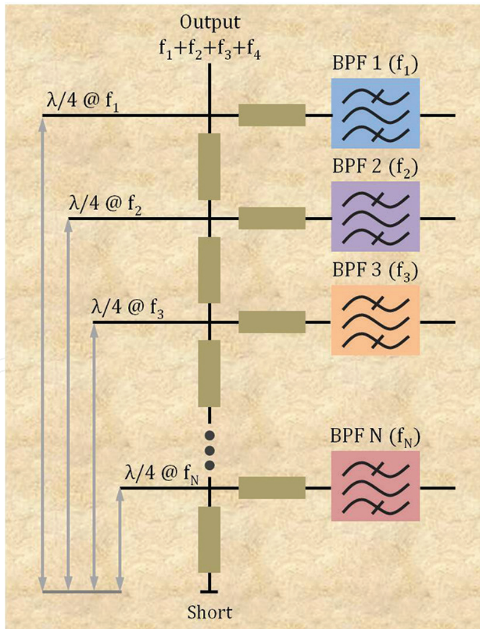
Figure 4. Frequency multiplexing network [23].
