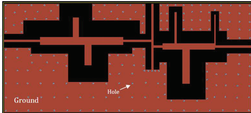
Figure 14. Layout of FDN for PCB.
