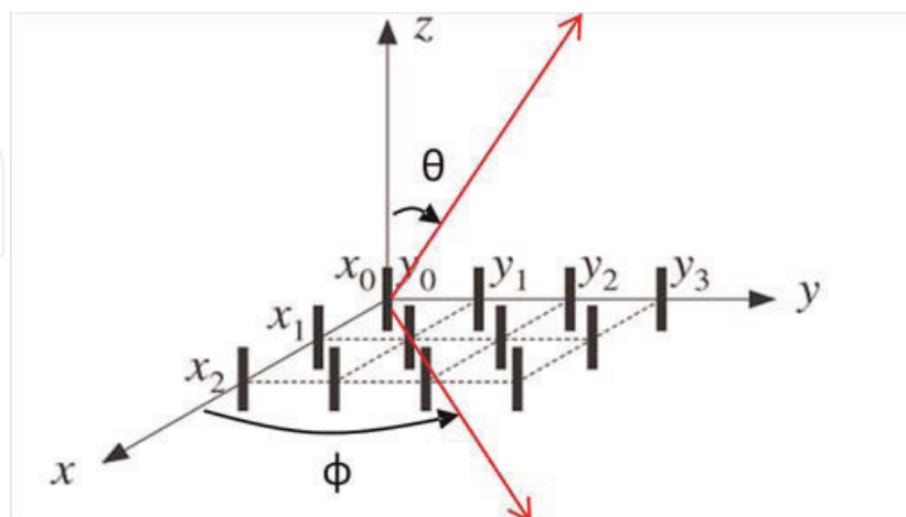
Figure 10. Two-dimensional array.
