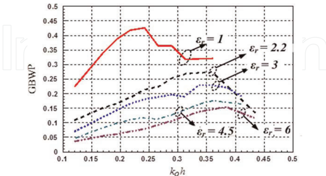
Figure 2. GBWP vs. k_0h . for different dielectric materials.
