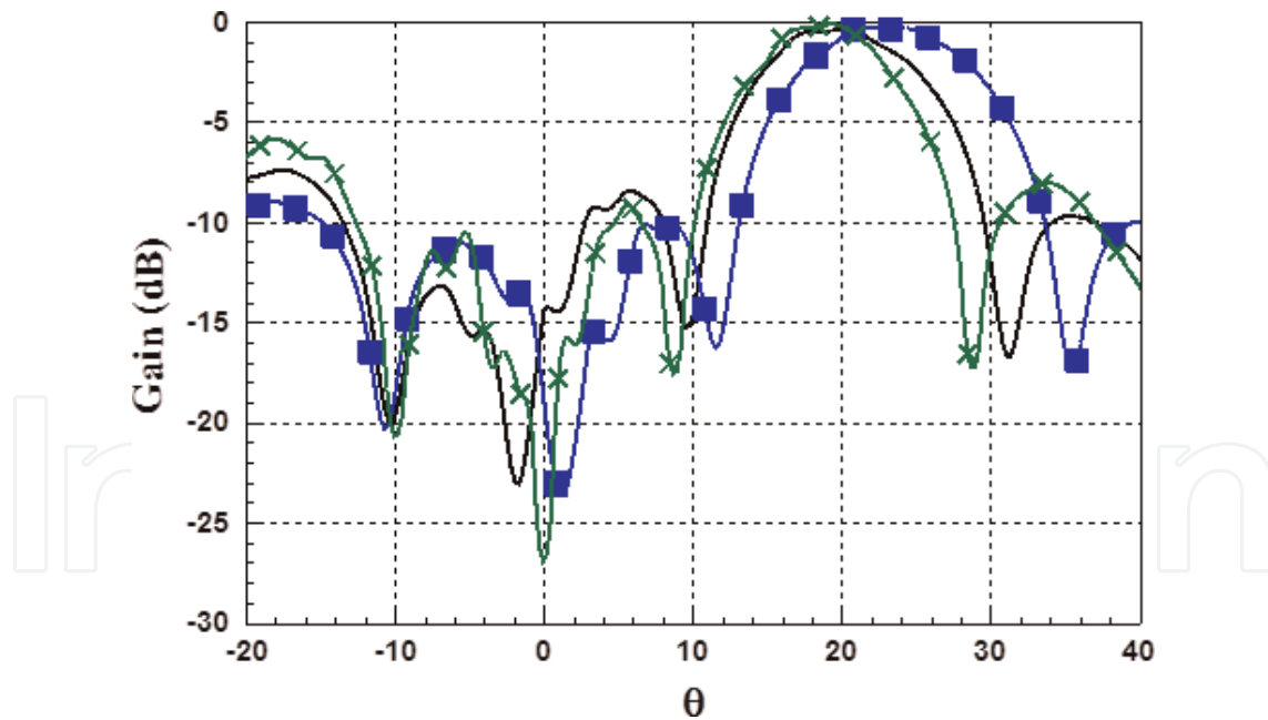
Figure 27. Radiation pattern of horizontally polarized full array in \varphi -plane ( \varphi=0^\circ cut) (— Measured @ 11.9 GHz, ■ Measured @ 10.8 GHz, × Measured @ 12.8 GHz).
