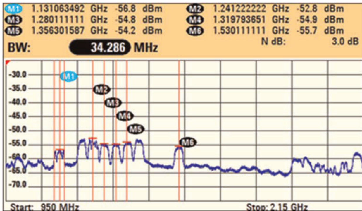
Figure 28. Spectrum analyser measurement of DBS signal.
