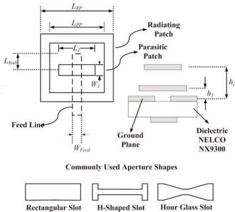
Figure 5. Aperture-coupled antenna and possible aperture shapes.
