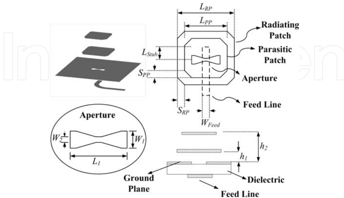
Figure 6. Aperture-coupled stacked microstrip patch antenna.
