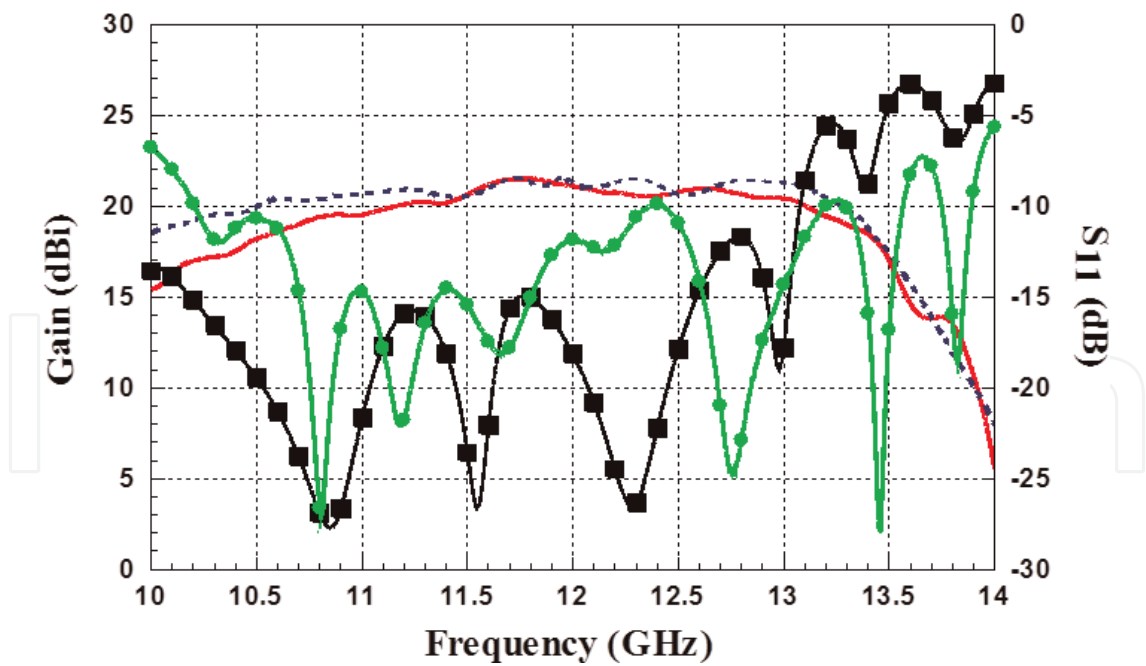
Figure 16. Input reflection coefficient and gain of 32 element subarrays ( — Measured Gain, - - Simulated Gain, ●●● Measured S11, ■■■ Simulated S11).
