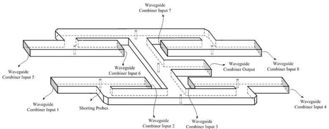
Figure 18. 8-to-1 power combiner.
