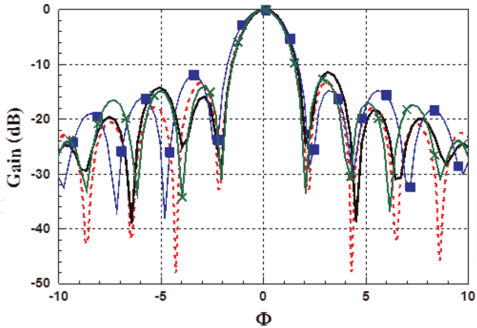
Figure 25. Radiation pattern of vertical polarized full array in azimuth plane ( \theta = 20^\circ cut). ( — Measured @ 11.9 GHz, - - Simulated @ 11.9 GHz, — Simulated @ 10.8 GHz, - - Measured @ 12.8 GHz).
