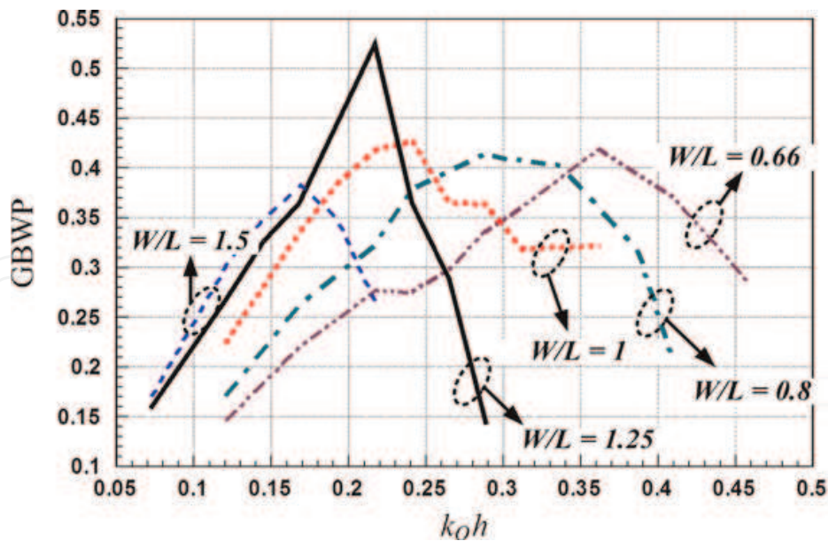
Figure 3. GBWP vs. k_0h for different aspect ratios.
