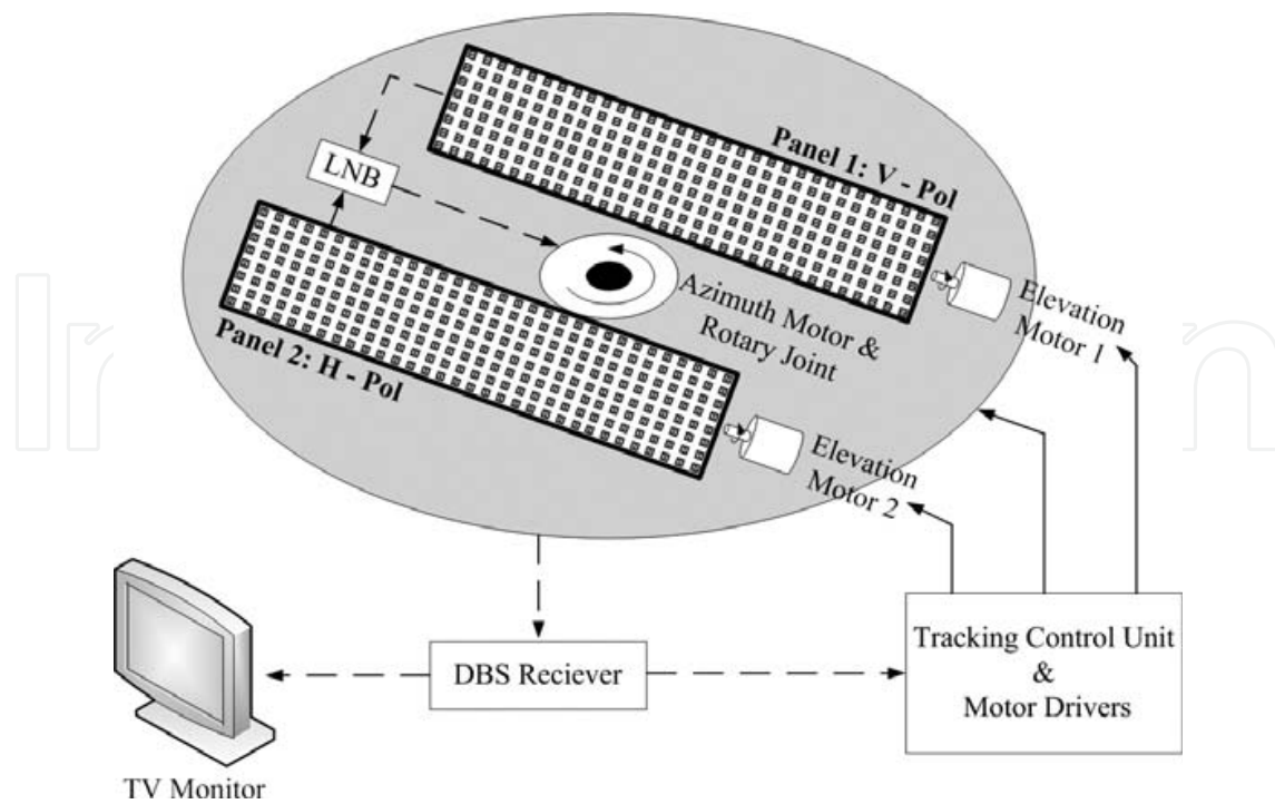
Figure 1. System configuration of the proposed array antenna.
