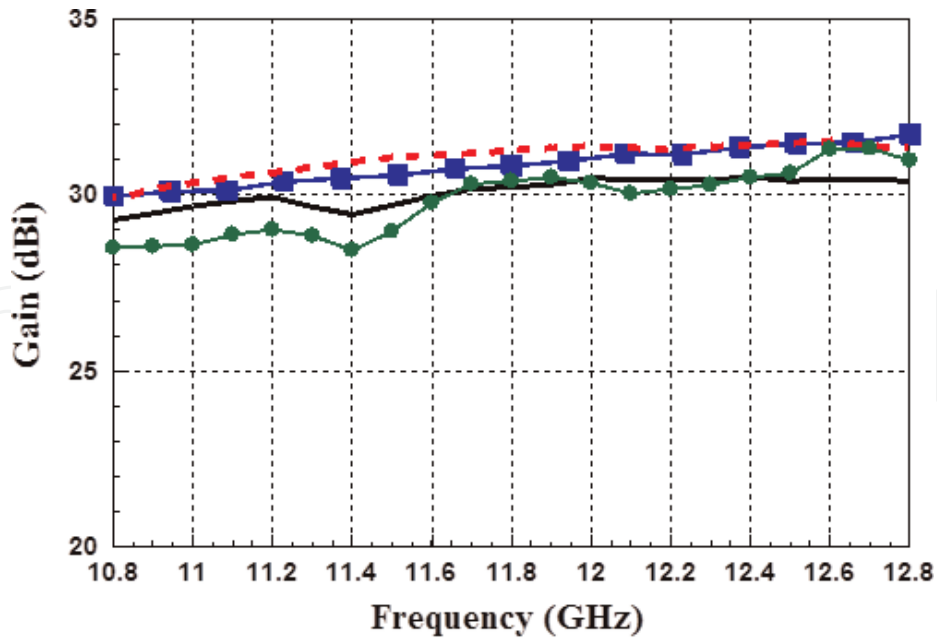
Figure 24. Gain of array antenna ( \theta = 20^\circ cut) ( — Measured Vertical Polarization, - - Measured Horizontal Polarization, - - Simulated 256 Element Array, — Simulated Reference).
