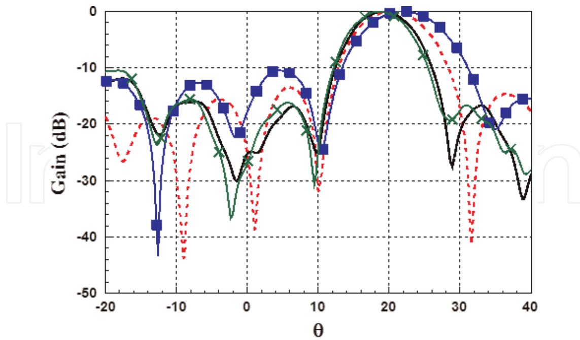
Figure 26. Radiation pattern of vertically polarized full array in \varphi -plane ( \varphi=0^\circ cut) (— Measured @ 11.9 GHz, - - - Simulated @ 11.9 GHz, ■ Measured @ 10.8 GHz, × Measured @ 12.8 GHz).
