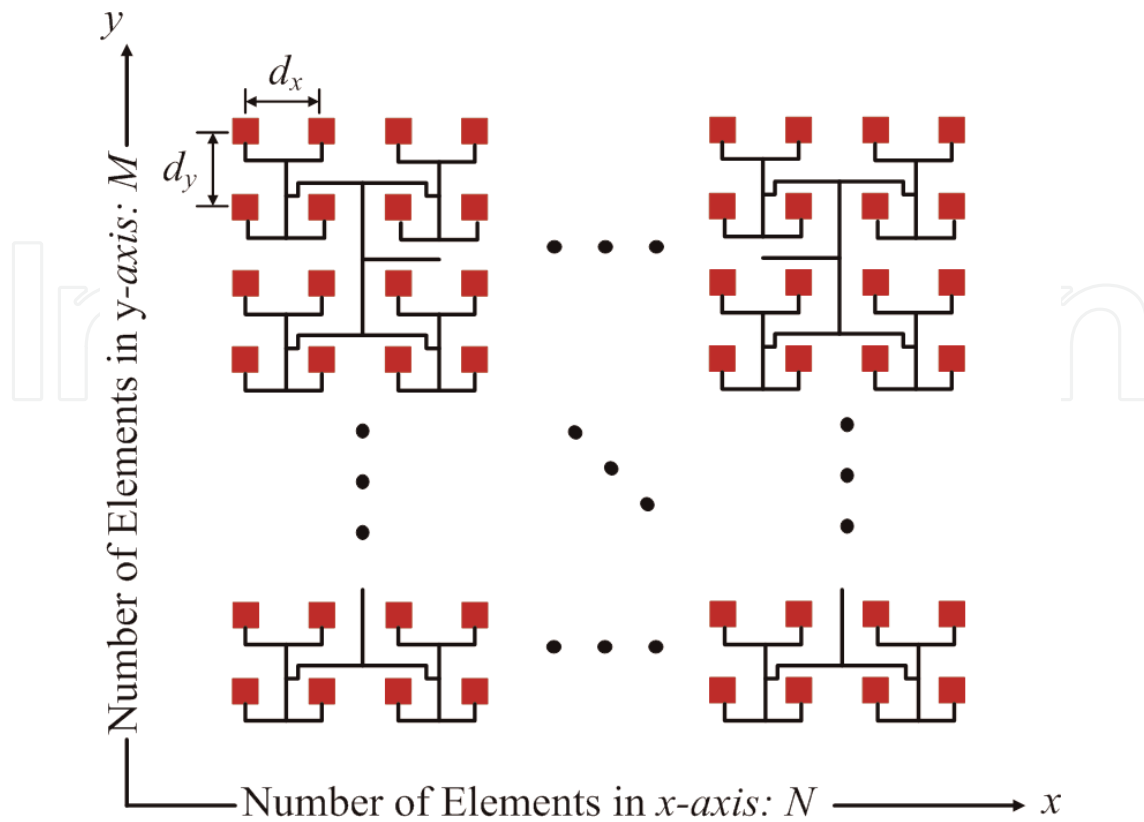
Figure 13. Layout of the feed network.
