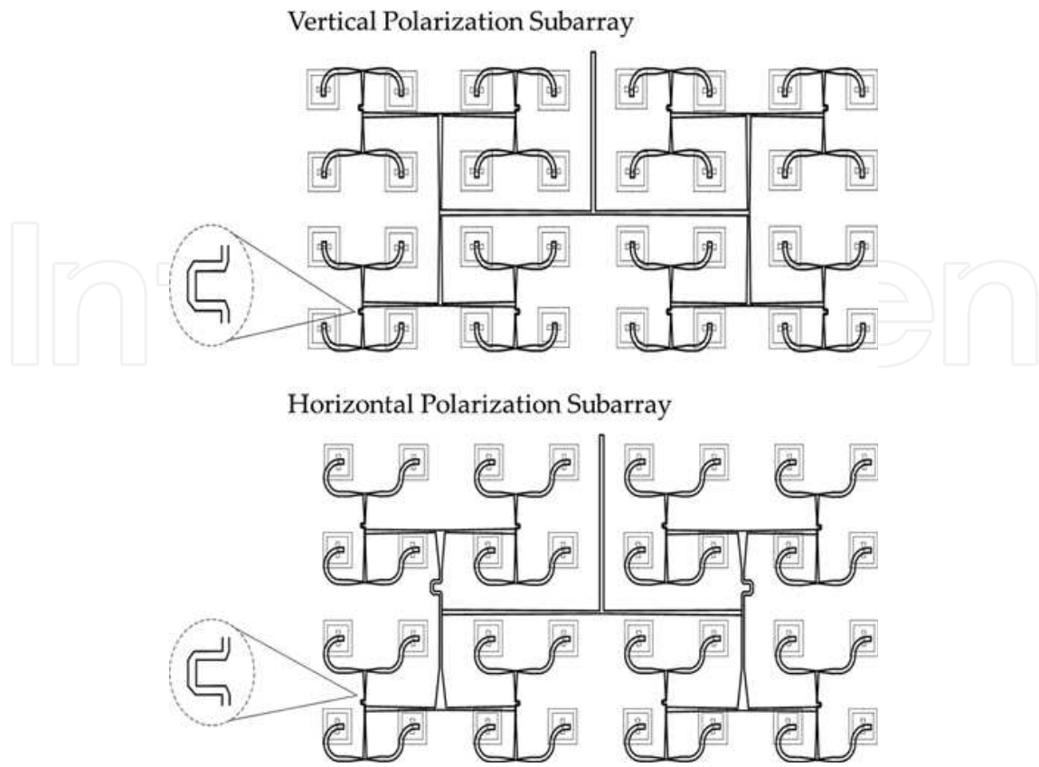
Figure 14. 32 element subarray configurations for vertical polarization and horizontal polarization.
