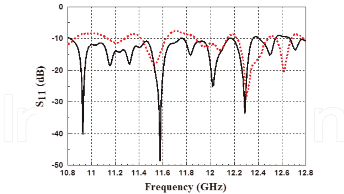
Figure 23. S11 of array antenna. ( — Measured, - - - Simulated).
