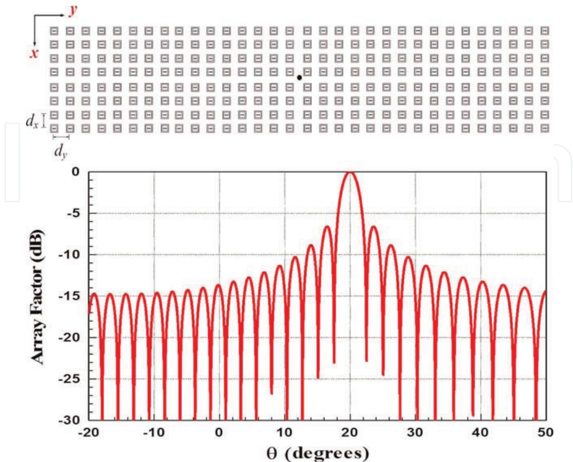
Figure 11. Array factor elevation pattern of synthesized array.
