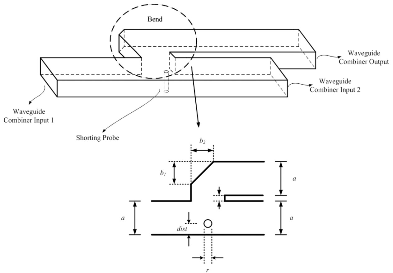
Figure 19. Waveguide bends and junctions.
