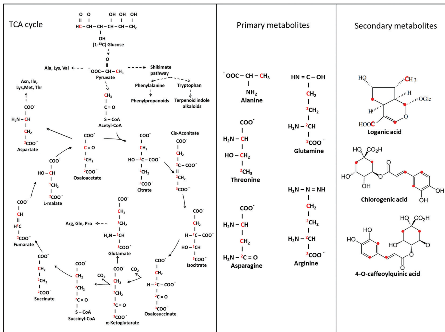
Figure 1. Label pattern of TCA cycle, amino acids, loganic acids, chlorogenic acid, and 4-O-caffeoyl quinic acid based on [1- 13 C] glucose feeding. Carbons and filled circles in red indicate 13 C-enriched positions.
