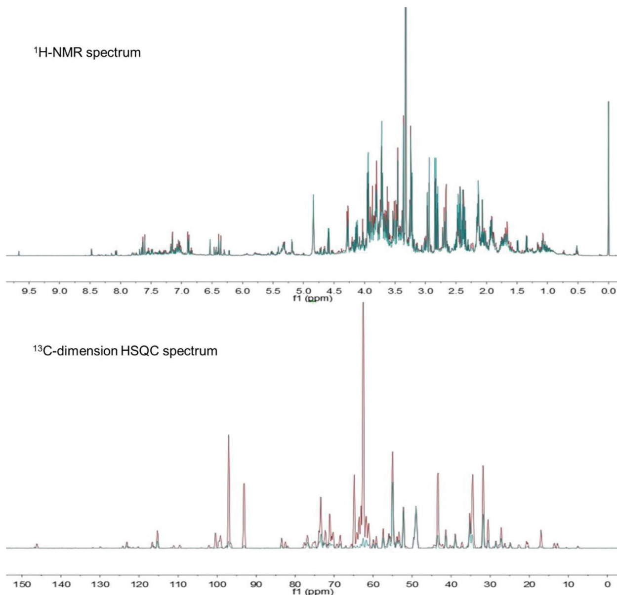
Figure 5. Superimposed ^1\text{H} NMR spectra and ^{13}\text{C} -dimension HSQC spectrum of labeled and non-labeled Catharanthus roseus plants. Spectra in green were non-labeled plants sample, spectra in red were ^{13}\text{C} -labeled plants sample.
