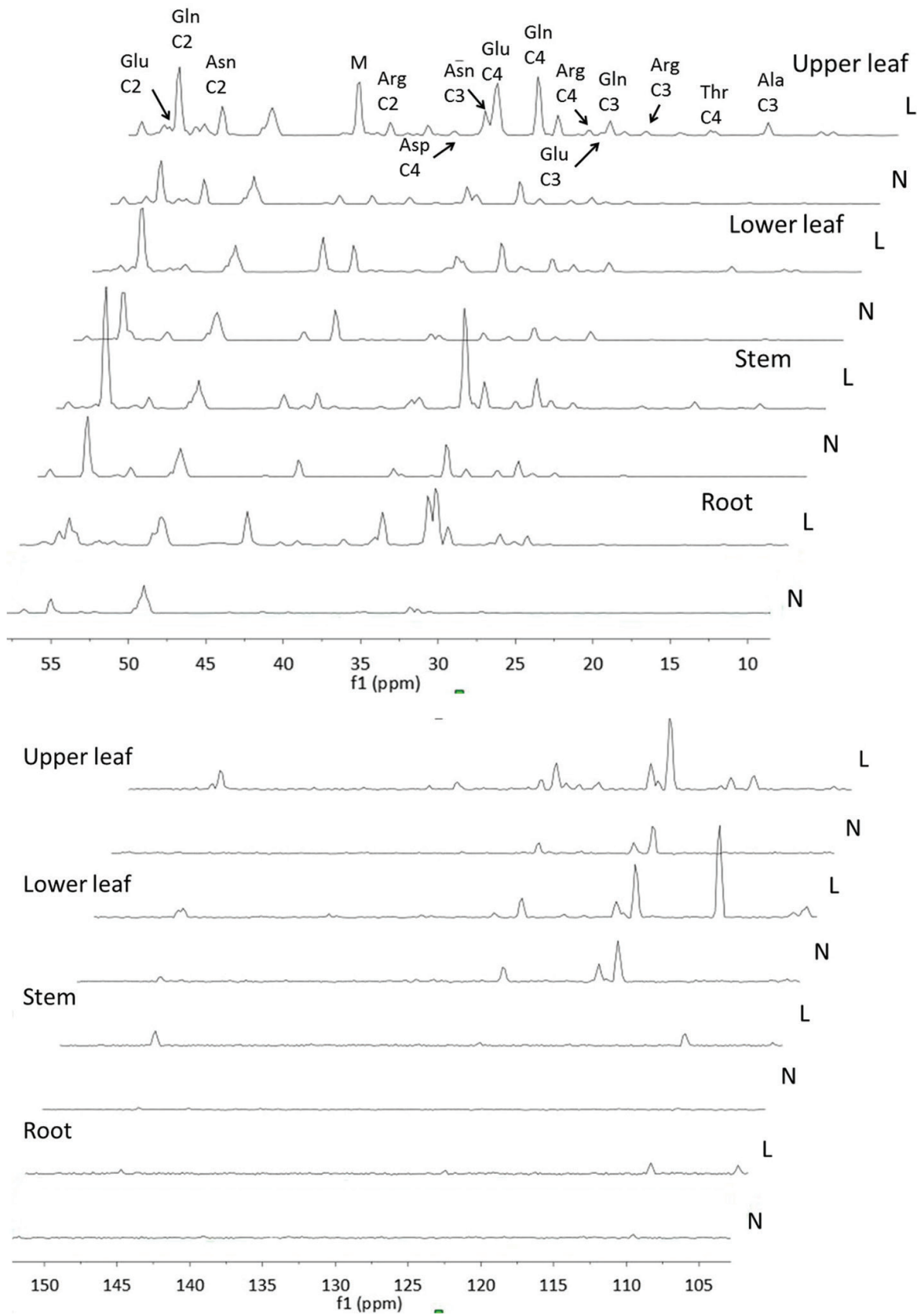
Figure 6. 13 C dimension of HSQC spectra of amino acids ( \delta 10–55 ppm) and secondary metabolites ( \delta 105–150 ppm) in different organs of Catharanthus roseus after feeding [ 1- 13 C ] glucose. L, labeled samples; N, non-labeled samples; M, malate.
