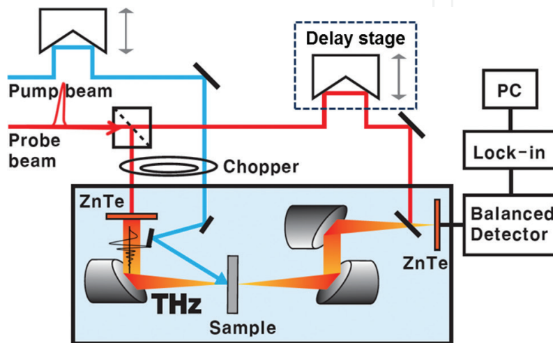
Figure 2. Schematic diagram of OPTP measurement system.
