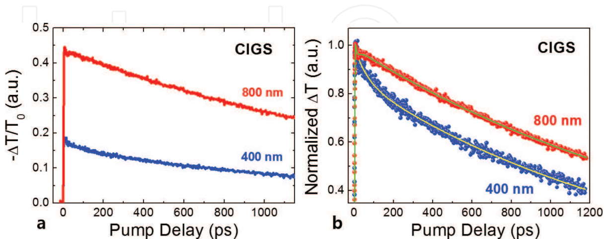
Figure 11. The measured -\Delta T/T spectra of the CIGS (a) and normalized \Delta T spectra of the CIGS (b) as a function of pump beam energies of 400 and 800 nm.
