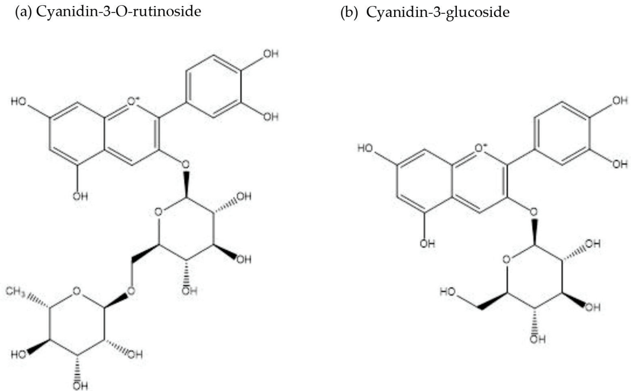
Figure 2. Chemical structures of the main anthocyanins found in açai and bacaba (a): 2-(3,4-dihydroxyphenyl)-5,7-dihydroxy-3-chromeniumyl-6- O -(6-deoxy- \alpha -L-mannopyranosyl)- \beta -D-glucopyranoside; (b): 2-(3,4-dihydroxyphenyl)-5,7-dihydroxy-3-chromeniumyl \beta -D-glucopyranoside [nomenclatures according to IUPAC].
