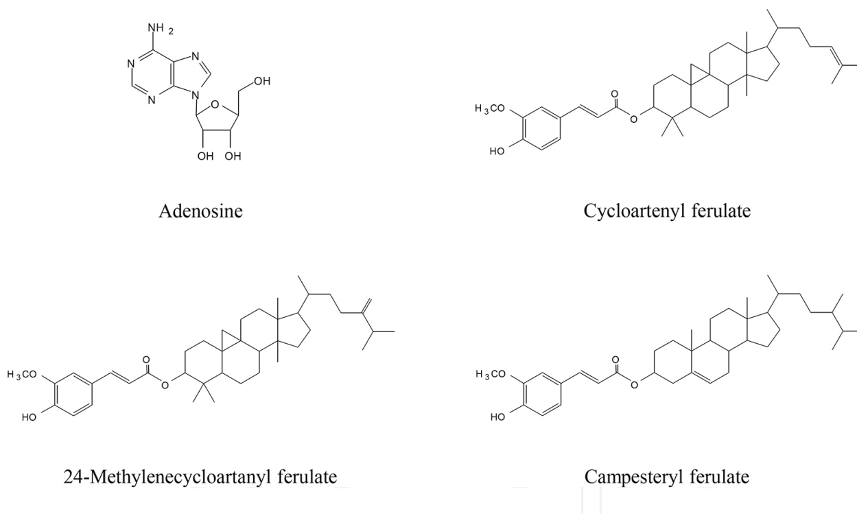
Figure 1. Chemical structure of bioactive components of rice bran.
