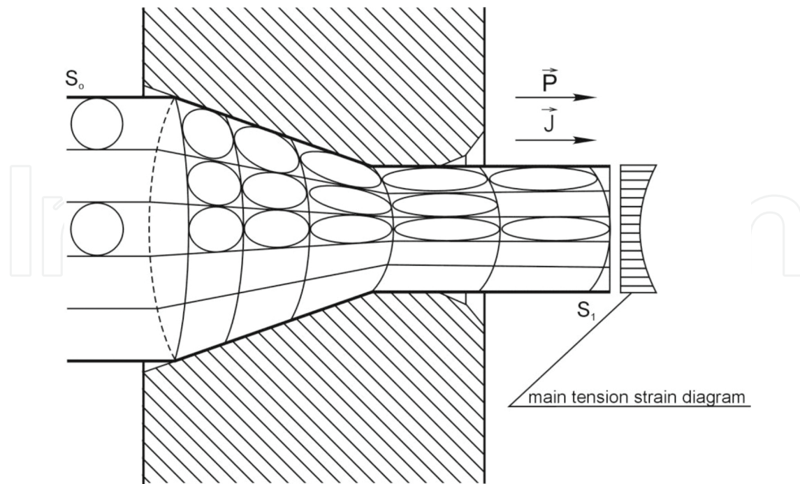
Figure 7. The perfect wire texture creation during electro-plastic wire dragging in condition of current density j and wire movement direction \vec{P} vector coexistence [26].
