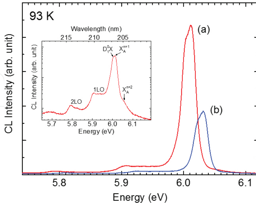
Figure 9. CL spectra of AlN grown under (a) Profile a and (b) Profile b using optimum LT-AlN BL T_g = 1050^\circ\text{C} .
