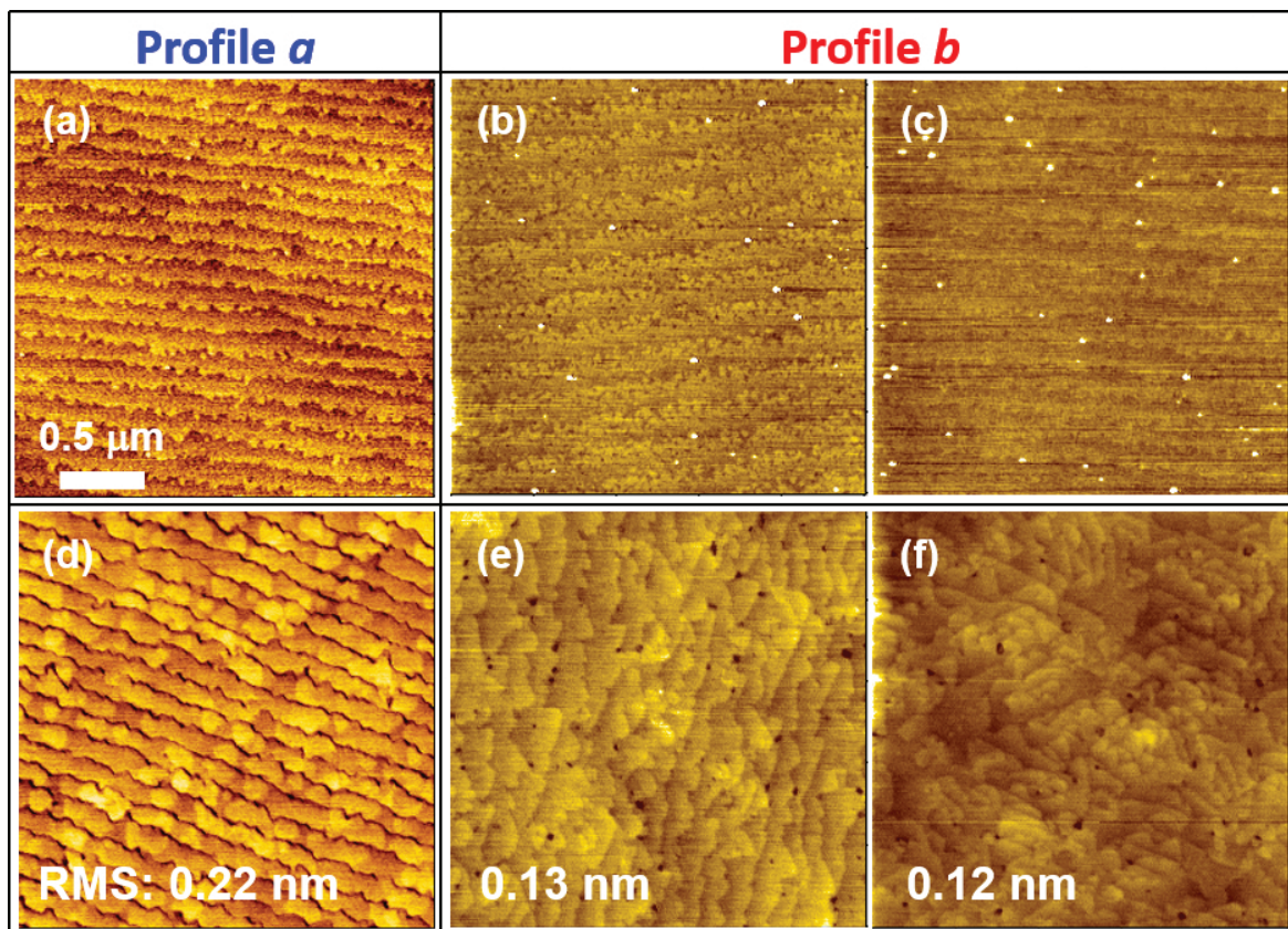
Figure 5. AFM surface morphologies of sapphire substrate after (a) thermal cleaning under Profile a , and before LT-AlN BL growth at (b) 1100°C and (c) 800°C under Profile b . The corresponding (d) HT-AlN growth for thermally cleaned substrate and under Profile b using (e) 1100°C and (f) 800°C LT-AlN BL T_g .
