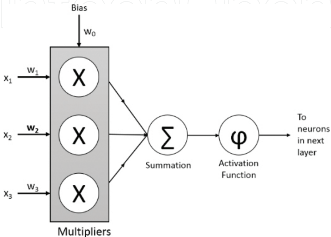
Figure 2. Mathematical model of a basic cell of artificial neural networks.
