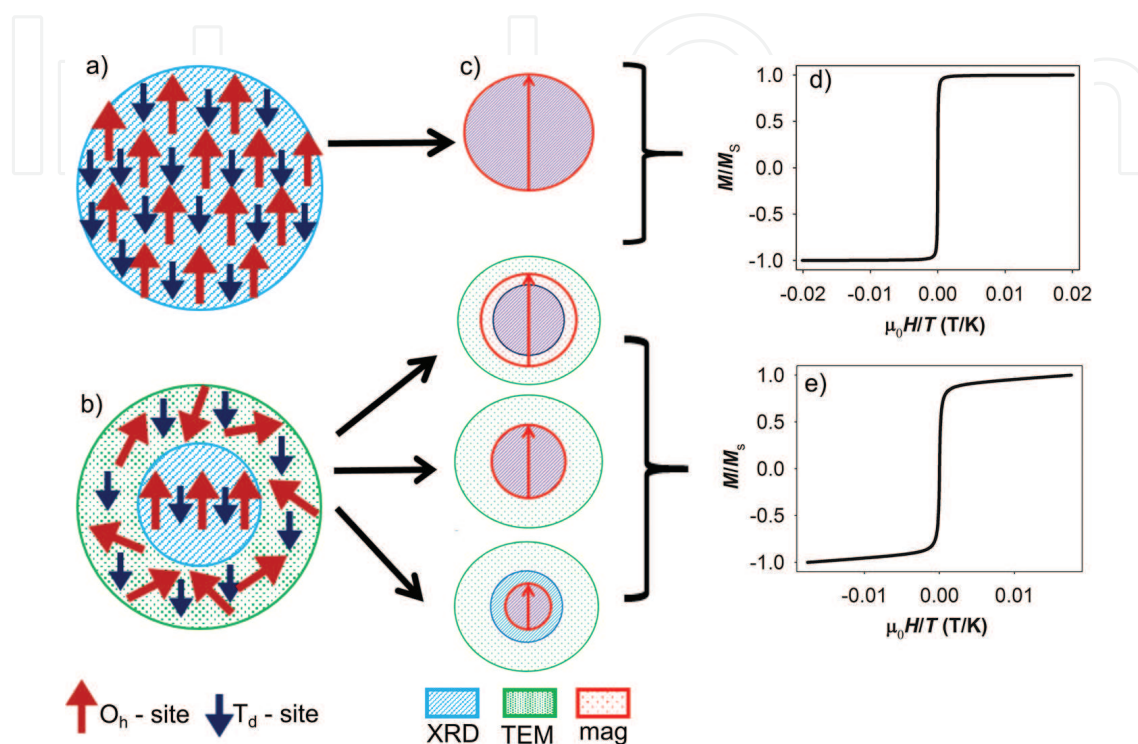
Figure 3. Scheme of the internal structure of ideal (a) and magnetic core-shell (b) structure of NP. (c) Scheme of the ideal and core-shell NP with the model of NP diameters determined by TEM, X-ray diffraction, and magnetic measurements. (d and e) Model Langevin curves for the ideal and core-shell NP with paramagnetic contribution due to the disordered spins in the NP shell.
