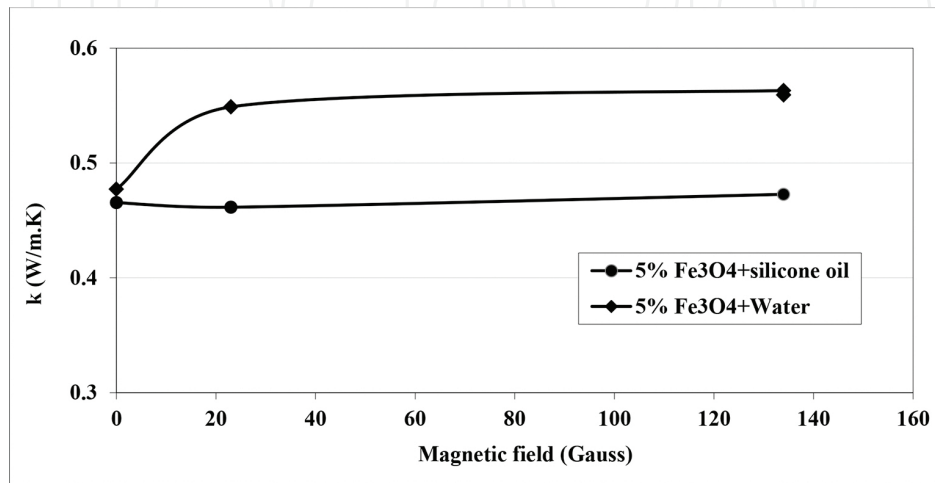
Figure 5. Thermal conductivity at 0–50°C interval and the temperature difference \Delta T = 20 K.
