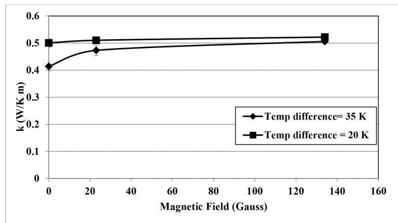
Figure 9. Temperature difference dependence of 20 vol% Fe 3 O 4 and silicone oil-based ferrofluid.
