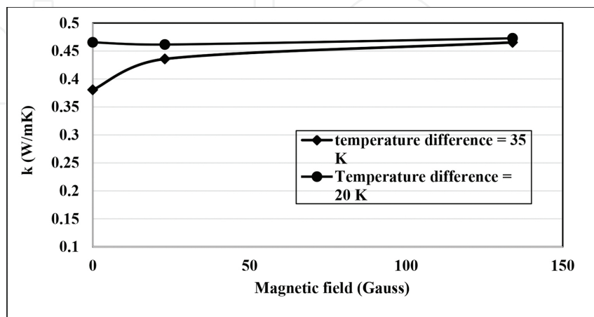
Figure 10. Temperature difference dependence of 5 vol% Fe 3 O 4 and silicone oil-based ferrofluid.
