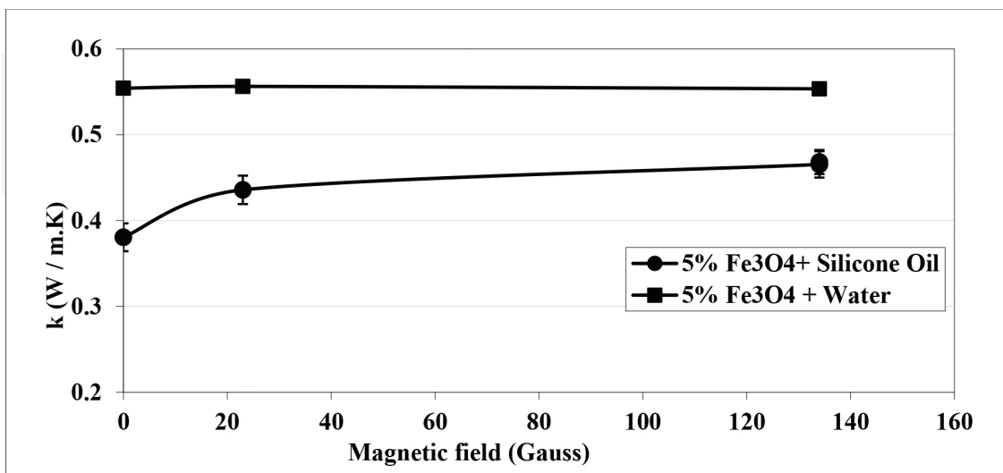
Figure 6. Thermal conductivity at 0–50°C interval and the temperature difference \Delta T = 35 K.
