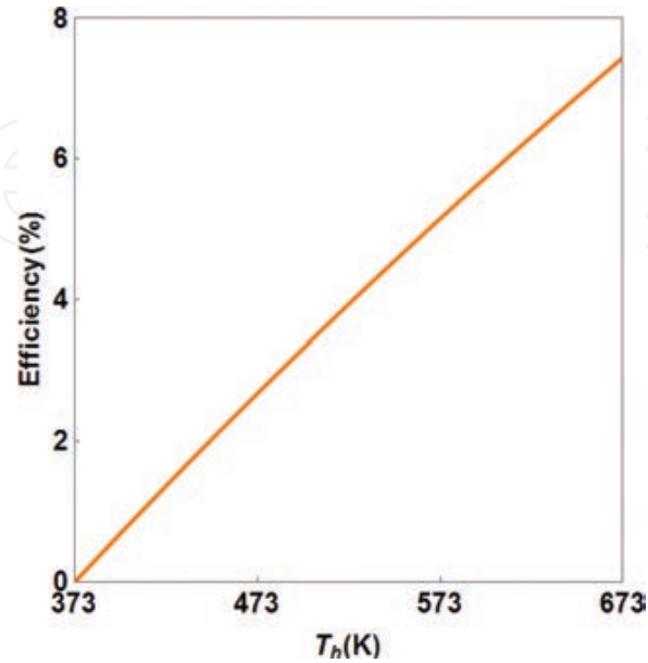
Figure 17. Efficiency of TEG as a function of hot-side temperature.
