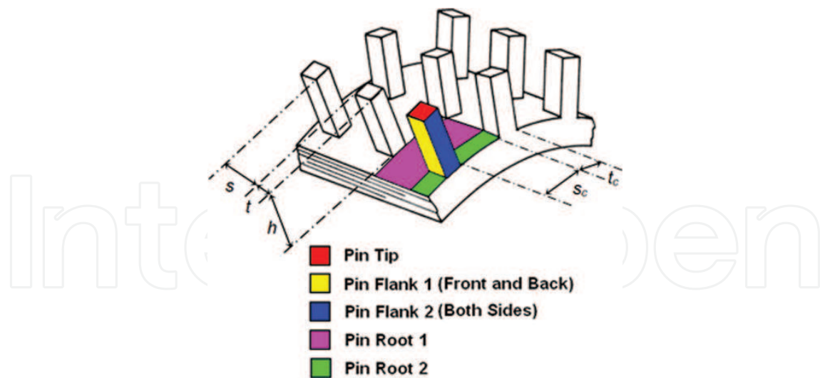
Figure 7. Schematic representation of pin-fin tube identifying five regions for heat transfer (after Ali and Briggs [2]).
