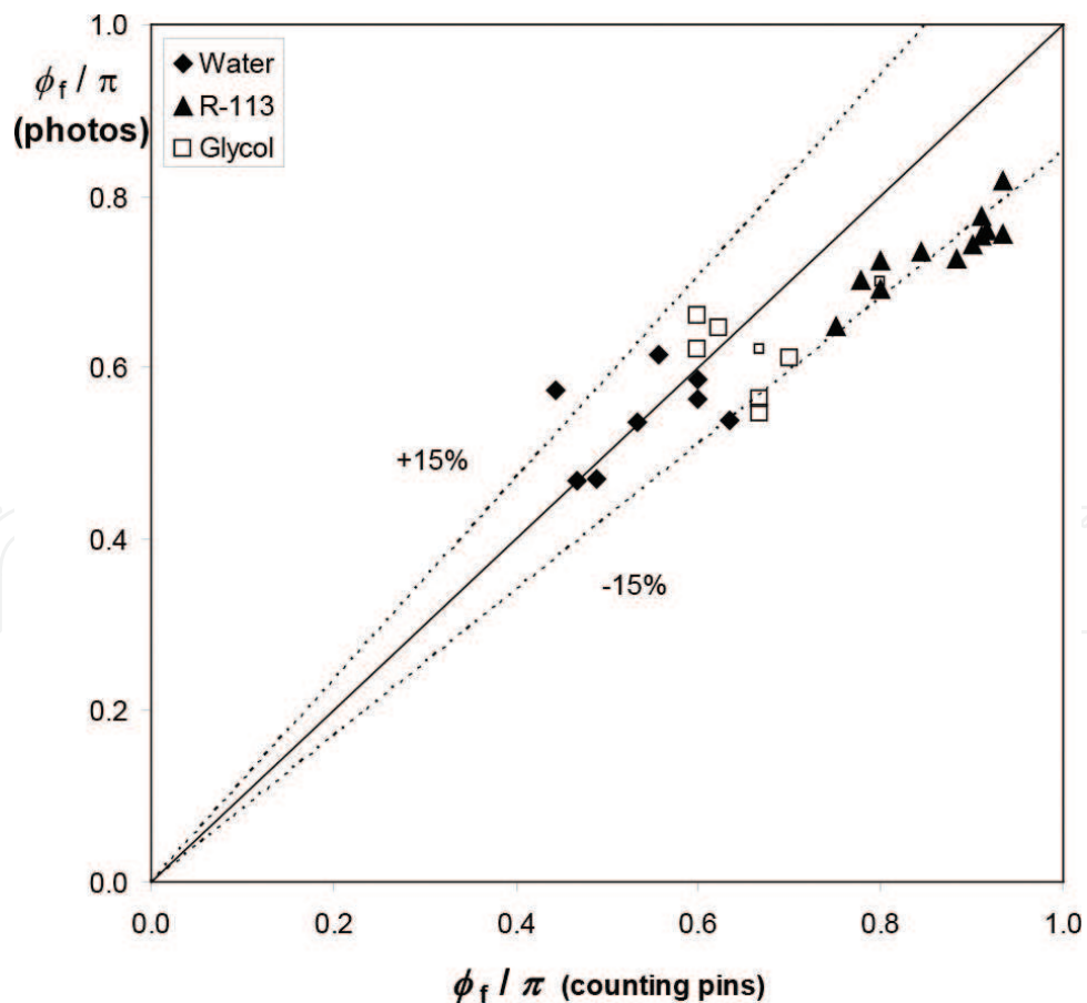
Figure 4. Comparison of pin-counting method with photographic method by Briggs [18].
