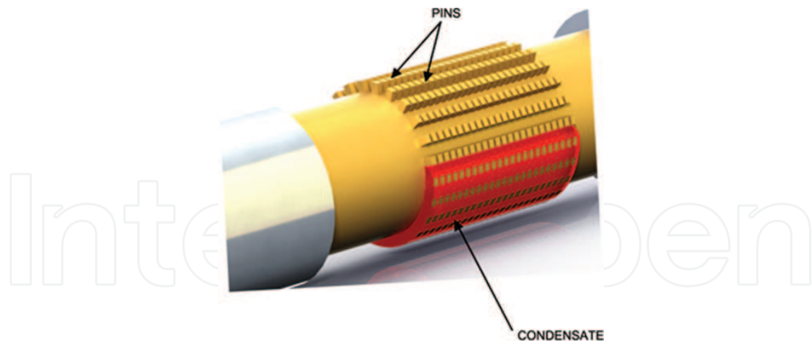
Figure 5. Sketch of a three-dimensional pin-fin tube.
