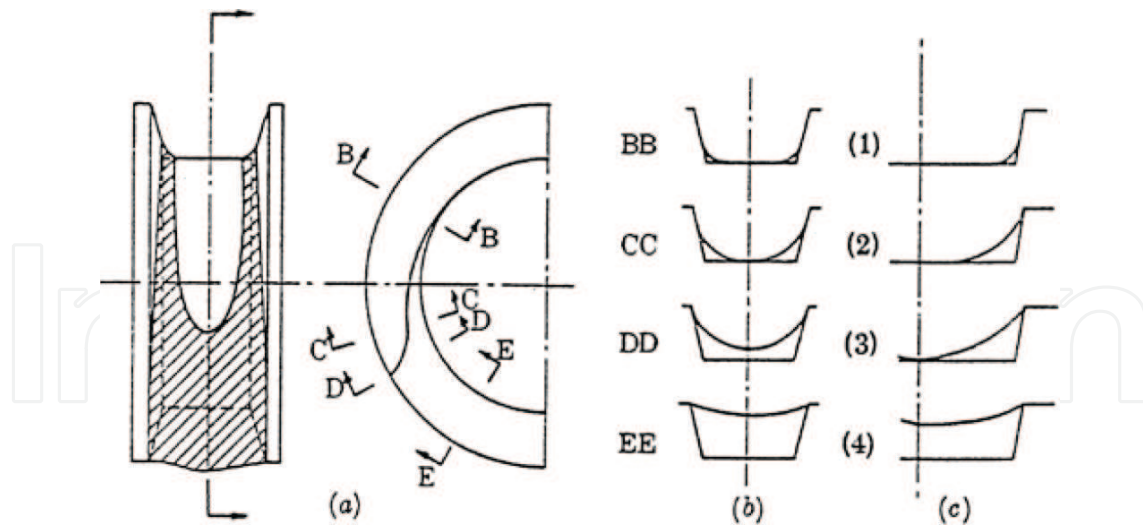
Figure 3. Configuration of retained liquid or condensate around a horizontal integral-fin tube. (a) Condensate retention on integral-fin tube. (b) Configuration of liquid around the narrow-spaced integral-fin tube. (c) Configuration of liquid around the wide-spaced integral-fin tube (after Masuda and Rose [15]).
