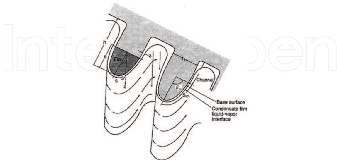
Figure 6. Fin parameters of vertical-fluted tube (after Gregorig [51]).
