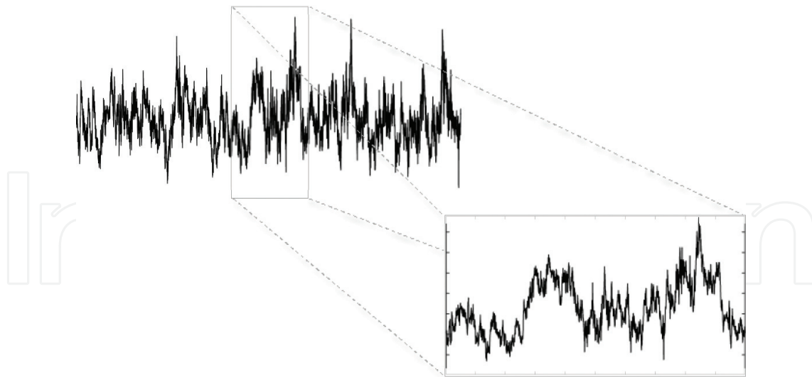
Figure 3. A portion of flow velocity u diluted in the box. This shows the statistical self-similarity features of flow velocity u .
