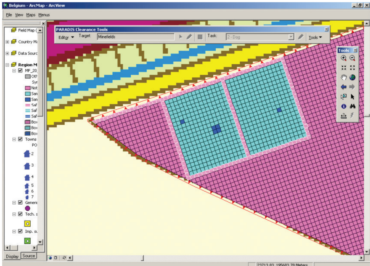
Figure 2. Mapping a square meter grid element on a minefield and following the status of each element as reported by the PDA users.
