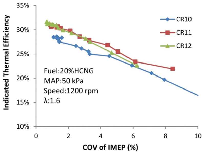
Figure 7. Variation in indicated thermal efficiency with COV of IMEP [35].
