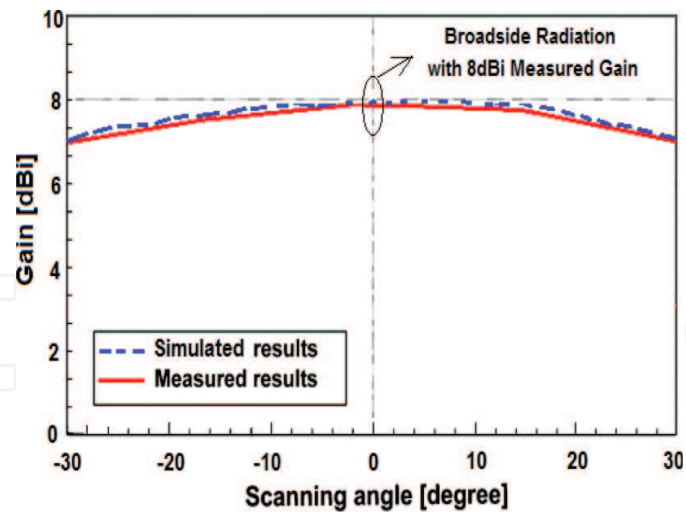
Figure 7. Gain curves versus scanning angle.
