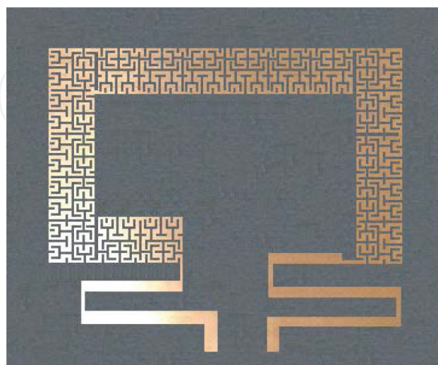
Figure 8. Fabricated Hilbert-curve loop RFID tag.
