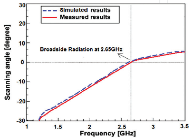
Figure 5. Scanning angle versus frequency. Broadside direction is 0°.
