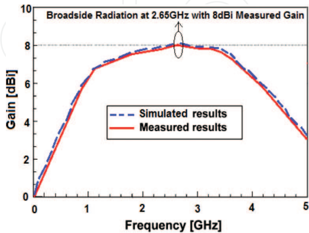
Figure 6. Gain as a function of frequency.
