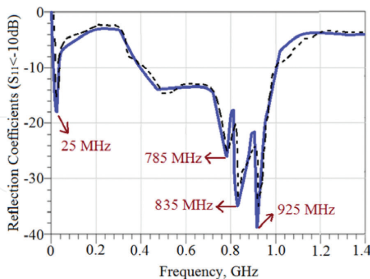
Figure 10. Simulated (solid-line) and measured (dashed-line) reflection-coefficient response.
