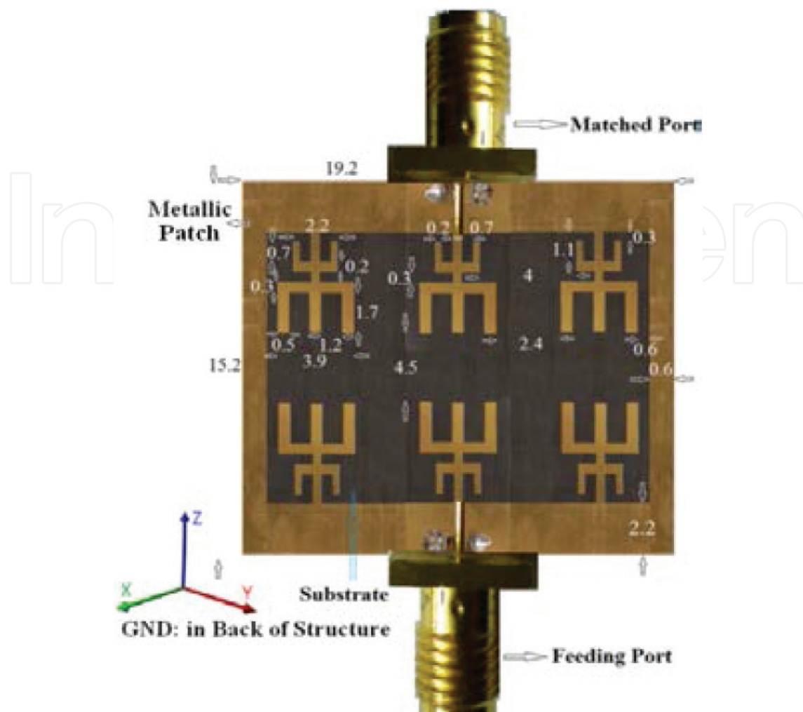
Figure 1. Fabricated prototype of the leaky-wave antenna (units in millimeters).
