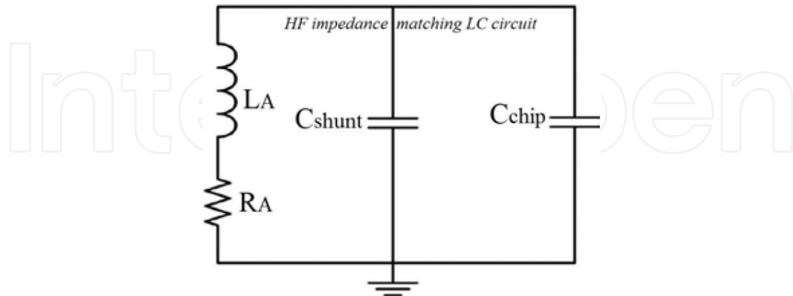
Figure 16. HF impedance-matching LC circuit.
