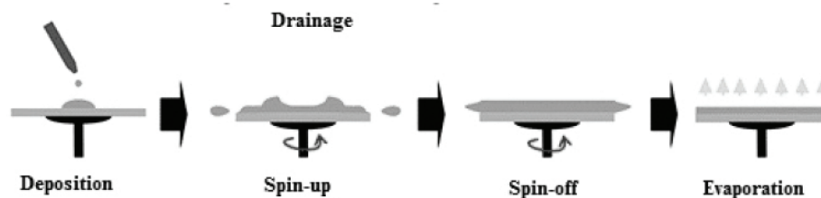
Figure 8. Spin-coating process.
