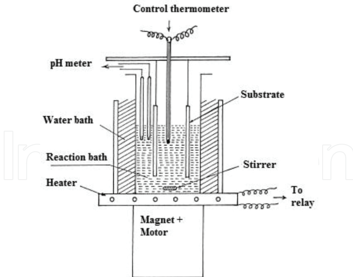
Figure 9. Home-made chemical bath deposition technique.
