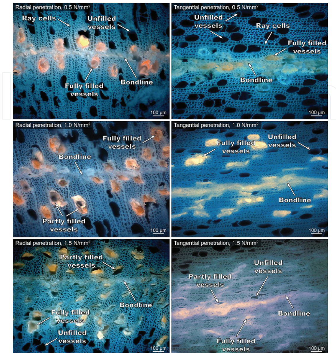
Figure 1. Example of epi-fluorescence microphotograph with the penetration of UF resin into poplar at three different pressures applied during the press cycle: 0.5 N/mm 2 , 1 N/mm 2 , and 1.5 N/mm 2 for radial and tangential penetration [2].
