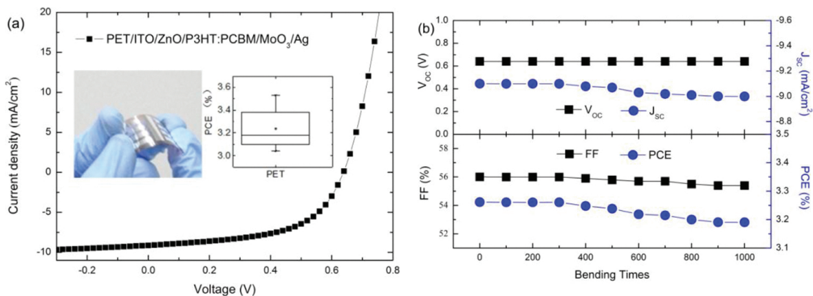
Figure 4. (a) Measured J-V characteristics of and PCE statistical result of flexible IOSCs. (b) Photovoltaic parameters as a function of the number of bending times up to 1000 cycles with a bending radius of about 50 mm [6]. Copyright (2015) The Japan Society of Applied Physics.
