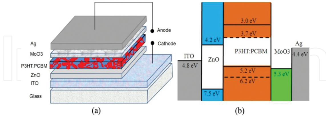
Figure 1. Schematic illustration and ideal energy diagram of materials for the inverted OSCs [6]. Copyright (2015) The Japan Society of Applied Physics.
