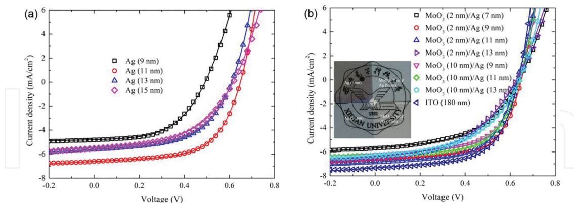
Figure 11. Measured (symbol) and calculated (solid line) J-V characteristics for OSCs fabricated on the (a) Ag or (b) MoO 3 /Ag anodes. Inset: A photograph of MoO 3 (2 and 10 nm)/Ag (9 and 11 nm) electrodes. Adapted with permission [11]. Copyright 2014, Elsevier.
