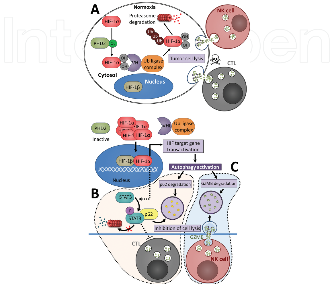
Figure 1. The role of hypoxic stress in the impairment CTL and NK-cell mediated lysis. (A) Under normoxia, the oxygen-sensitive prolyl hydroxylase domain protein 2 (PHD2) hydroxylates HIF-1 \alpha subunit. Hydroxylated HIF-1 \alpha interacted with Von Hippel-Lindau protein (VHL), subjected to ubiquitination and subsequently degraded by the ubiquitin-proteasome system. Under hypoxic stress, the function of PHD2 protein is blocked, HIF-1 \alpha is therefore stabilized and translocated to the nucleus to form heterodimeric complex with HIF-1 \beta to transcriptionally induce the expression of HIF-target genes involved in several pathways such as autophagy. (B) Under hypoxia, STAT3 is phosphorylated at Ser-705 residue in a HIF-dependent manner by a mechanism which is not fully understood. (C) The hypoxia-dependent induction of autophagy leads to the degradation of the adaptor protein p62/SQSTM1, involved in targeting phospho-STAT3 to the ubiquitin proteasome system for degradation. Thus, targeting autophagy accumulated p62/SQSTM1 and therefore accelerated the degradation of phospho-STAT3. The degradation of phospho-STAT3 restores CTL-mediated lysis of tumor cells. In addition, the induction of autophagy in hypoxic tumor cells leads to the selective degradation of granzyme B (GZMB), a serine protease released by natural killer (NK) cells and contained in the cytotoxic granules. Such degradation inhibits NK-mediated lysis of tumor cells.
