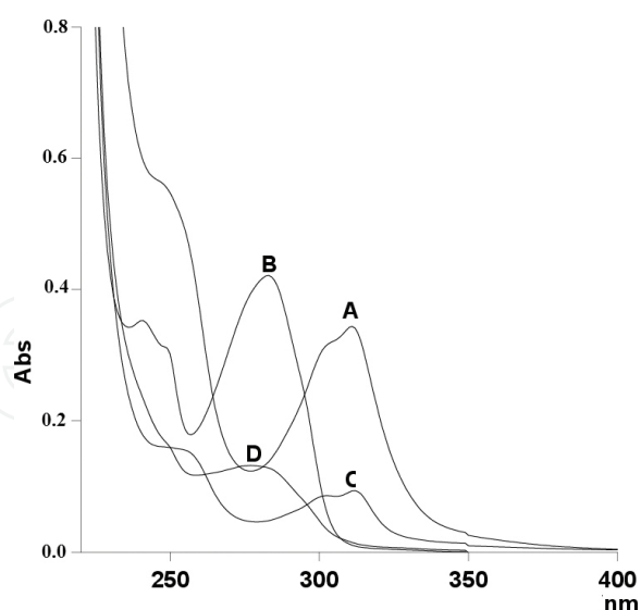
Figure 3. UV-Vis spectra of (A) Pd(OAc) 2 (BipyOH), (B) BipyOH, (C) Pd(OAc) 2 L 7 , and (D) L 7 .
