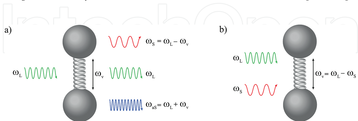
Figure 1. Schematic showing the stimulated Raman-scattering process. The molecules in the Raman-active medium are described by harmonic oscillators of frequency \omega_v . The incoming laser beam has frequency \omega_L . (a) Modulation of the refractive index and subsequent emission of Stokes and anti-Stokes radiation and (b) beating of the Stokes frequency with the laser field reinforcing the vibrational oscillation of the molecule.
