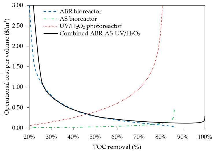
Figure 4. Comparison of operational costs per cubic meter of treated actual slaughterhouse wastewater using individual ABR, AS, and UV/H 2 O 2 processes and the combined ABR-AS-UV/H 2 O 2 system.
