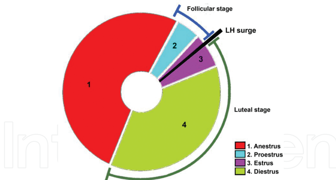
Figure 1. Schematic representation of the standard canine estrous cycle. Adapted with permission from [12].
