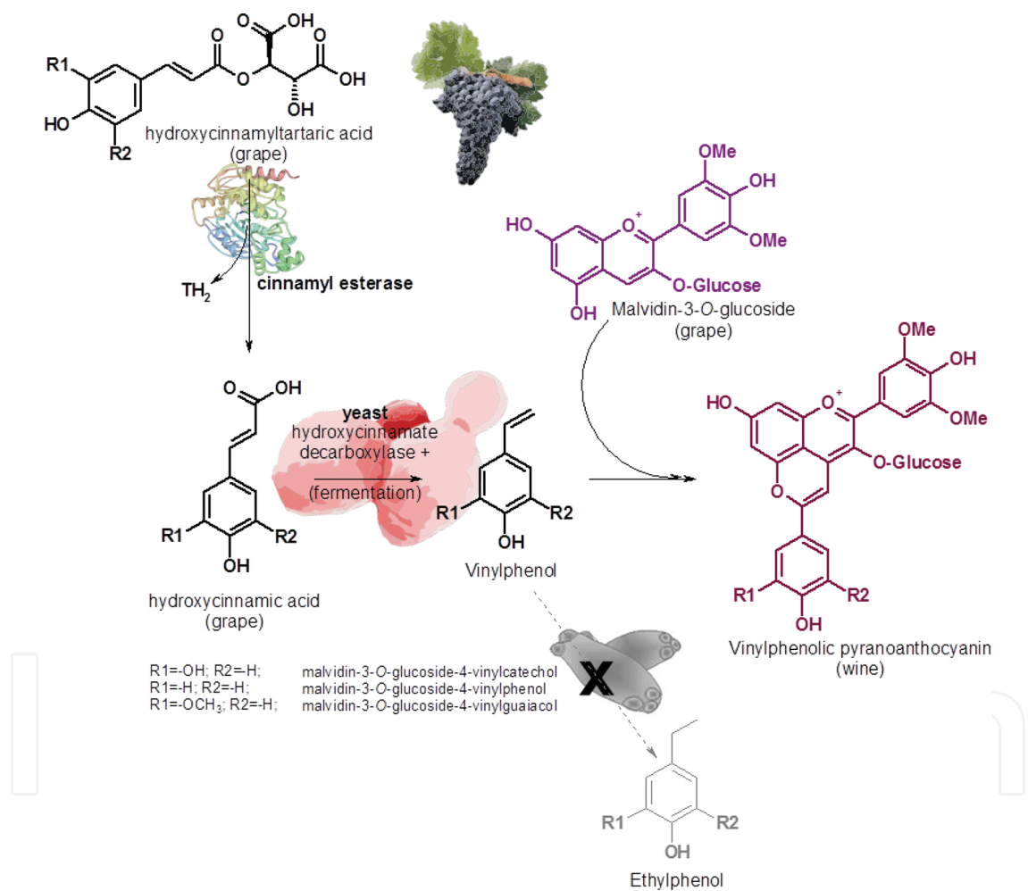
Figure 10. Mobilization of TE-HCAs to form stable VPAs decreasing the amount of 4-ethylphenol precursors during fermentation.
