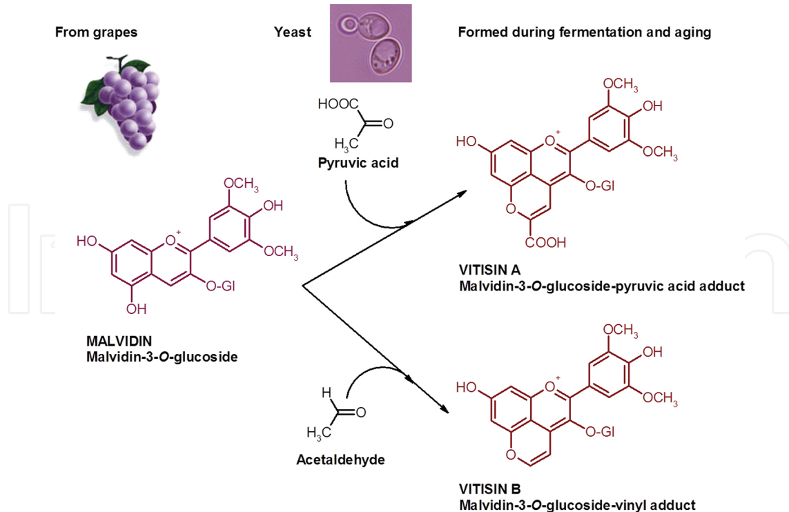
Figure 2. Formation of vitisins A and B by chemical reaction between malvidin and pyruvic acid or acetaldehyde, respectively.
