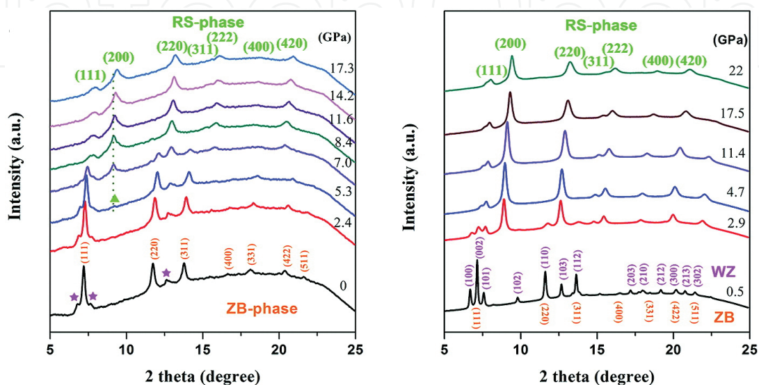
Figure 5. High-pressure XRD patterns of \beta -MnS NCs (left) and \gamma -MnS bipods with \beta -MnS core (right). Legend: RS = \alpha -MnS, ZB = \beta -MnS, WZ = \gamma -MnS. The stars and triangle in the left panel represent diffraction peaks from \gamma -MnS and the (200) peak of \alpha -MnS, respectively. Adapted with permission from [40]. Copyright (2012) American Chemical Society.
