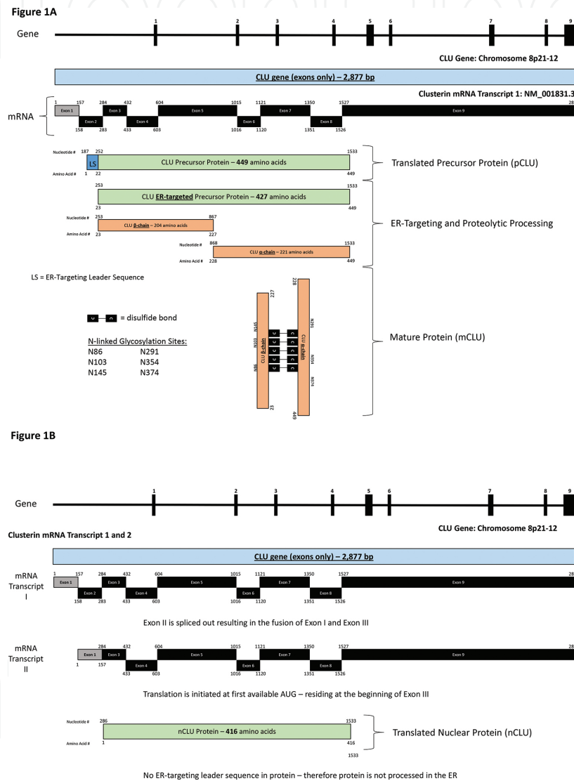
Figure 1. CLU transcription and translation. In humans, CLU is a single-copy gene located on the short arm of chromosome 8 that is comprised of nine exons spanning approximately 2.8 kb. (A) The mCLU isoform is generated from mRNA transcript 1 from a canonical translational start site in exon 2. The resulting precursor protein (pCLU), which contains an N-terminal ER-targeting leader sequence (LS), is transported to the ER where the 22-amino-acid LS is removed. CLU is then cleaved into the alpha and beta subunits and rapidly disulfide bonded and glycosylated to form an anti-parallel, heterodimeric glycoprotein: mCLU. (B) Alternatively, the nCLU isoform is generated from mRNA transcript 2. In this transcript, a splicing event removes exon 2 resulting in the fusion of exons 1 and 3. Translation is initiated at the beginning of exon 3 resulting in a truncated CLU isoform that lacks the ER-targeting LS. Therefore, the nCLU isoform, which retains the nuclear localization sequence, bypasses the ER/Golgi apparatus and is shuttled between the cytosol and the nuclear compartment.
