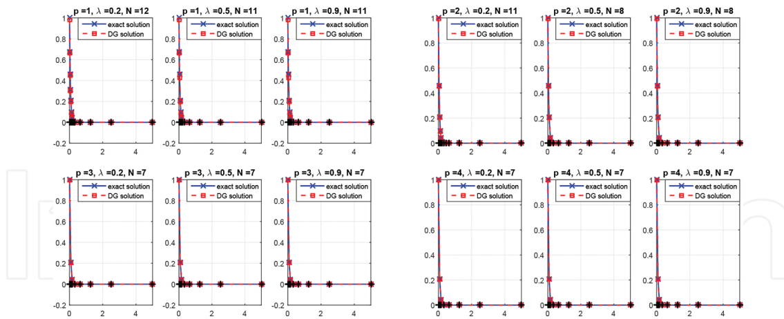
Figure 7. u , u_h , and final meshes for Example 7.2 with \beta = -20 using P^p , p = 1 to 4, and Tol = 10^{-2} .
