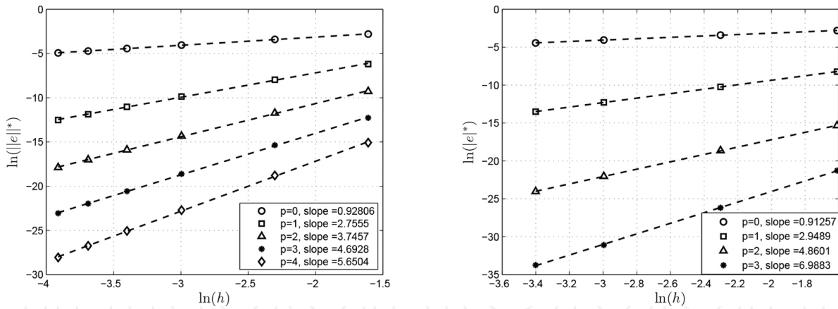
Figure 2. Log-log plots of \|e\|^* (left) versus h for Example 7.1 using N = 5, 10, 20, 30, 40, 50 and P^p, p = 0 to 4. Log-log plots of |e|^* (right) versus h using N = 5, 10, 20, 30 elements using P^p, p = 0 to 3.
