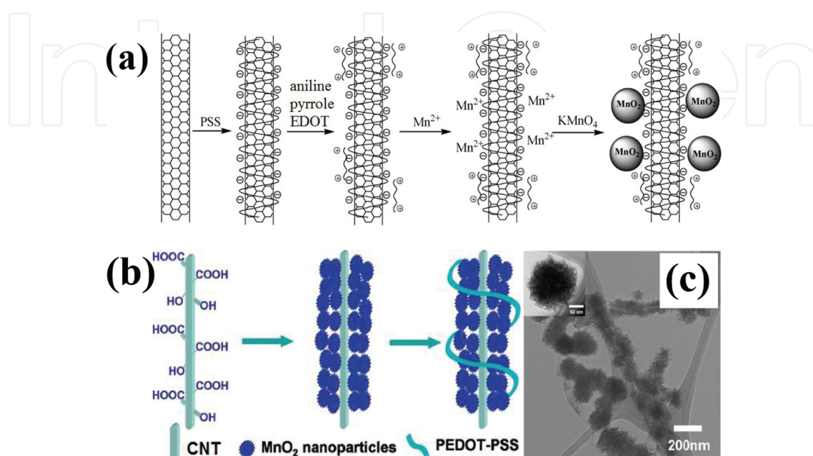
Figure 6. (a, b) Schematic illustration of synthesizing \text{MnO}_2 /conducting polymers on CNTs-PSS. (c) TEM image of \text{MnO}_2 /PEDOT/CNTs.
