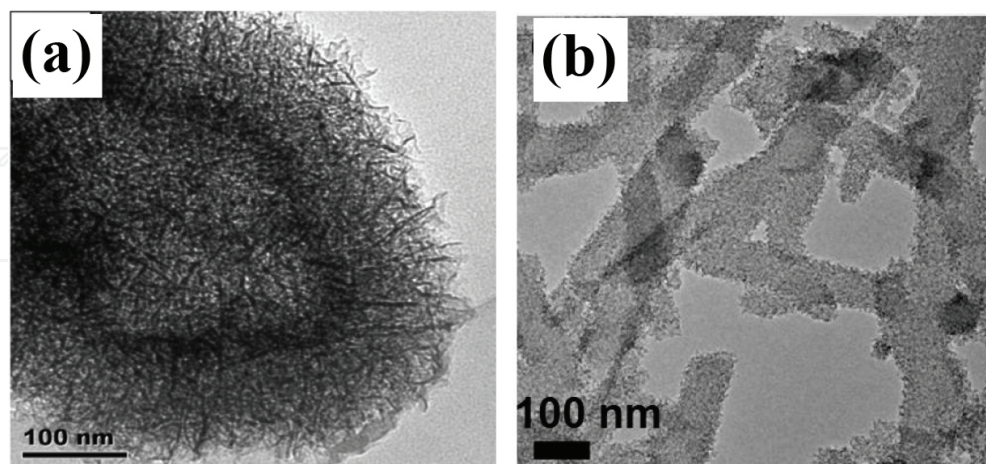
Figure 5. TEM images of MnO 2 /PANi (a) hollow spheres and (b) nanofibers.
