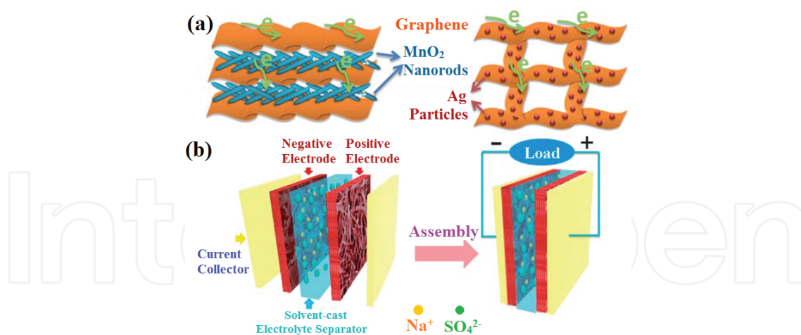
Figure 7. Illustrations of (a) MnO 2 /graphene and graphene/Ag freestanding films and (b) the as-fabricated asymmetric supercapacitor devices.
