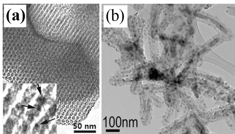
Figure 4. (a) TEM images of MnO 2 /CMK-3. (b) TEM image of highly graphitic carbon-tipped MnO 2 /mesoporous carbon/MnO x hybrid nanowires.
