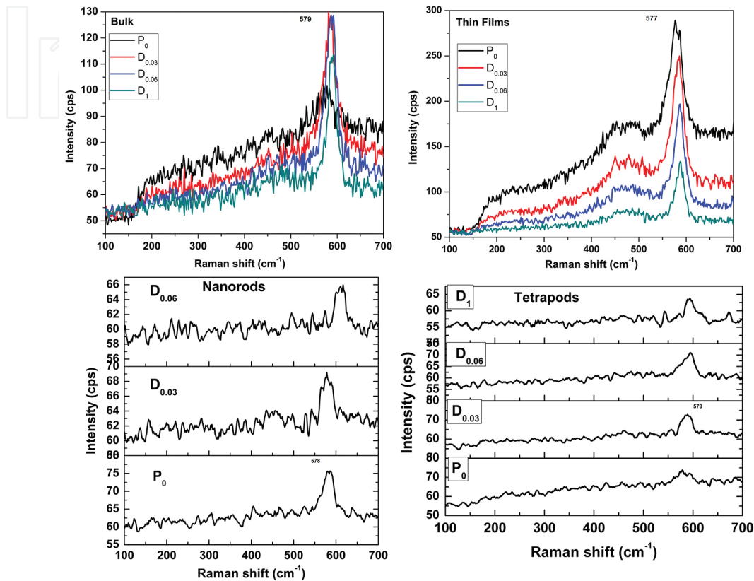
Figure 10. Raman spectrum of ZnO material with 325 nm excitation source for bulk, thin films, rods and tetrapods.
