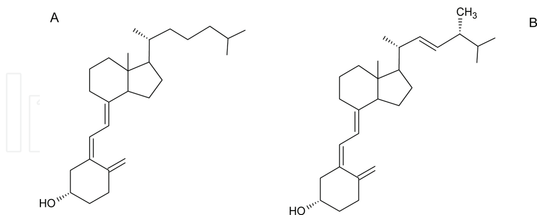
Figure 2. Chemical structures of (A) cholecalciferol and (B) ergocalciferol (drawn in ACD/ChemSketch®).
