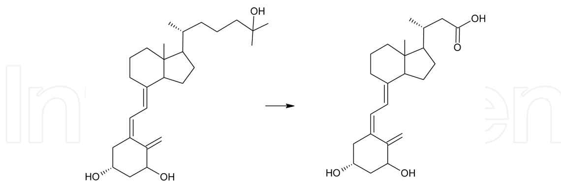
Figure 5. Image illustrating the inactivation of calcitriol, through conversion in calcitroic acid (drawn in ACD/Chem-Sketch®).
