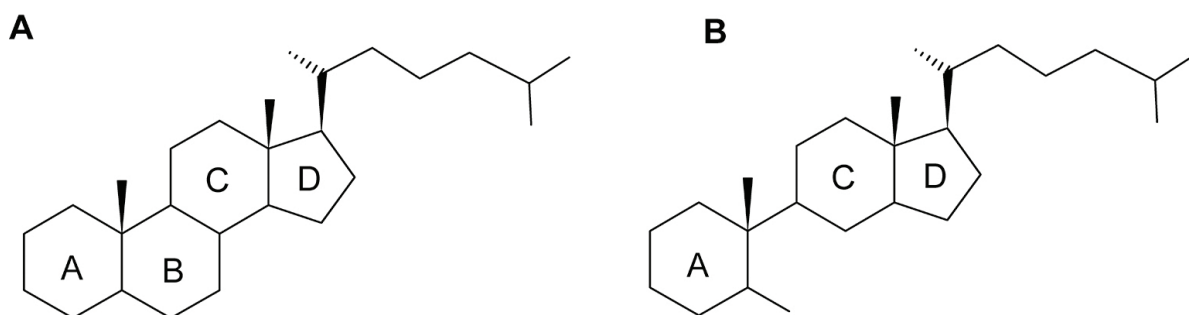
Figure 1. General chemical structures of (A) steroid and (B) seco-steroid (drawn in ACD/ChemSketch®).
