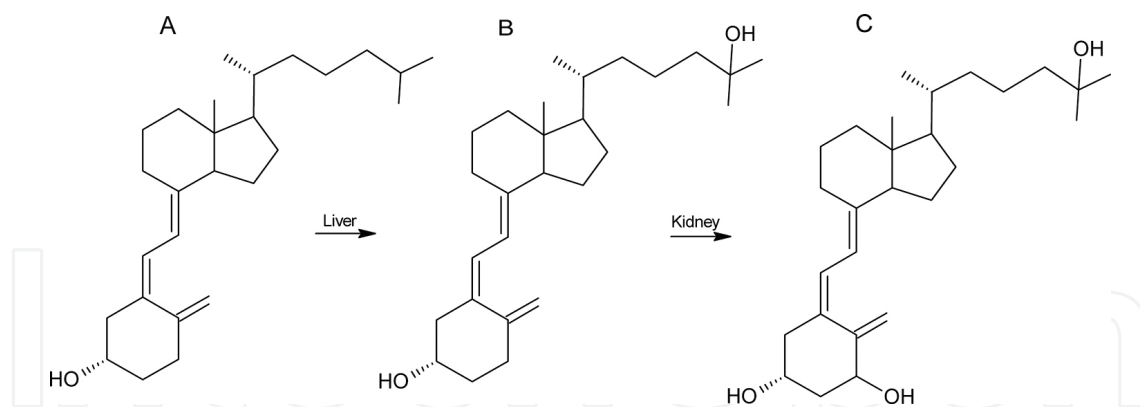
Figure 4. Representation of cholecalciferol three different chemical structures: (A) calcio, (B) calcidiol, and (C) calcitriol. This scheme also represents the overall chemical reactions involved in vitamin D activation (drawn in ACD/Chem-Sketch®).
